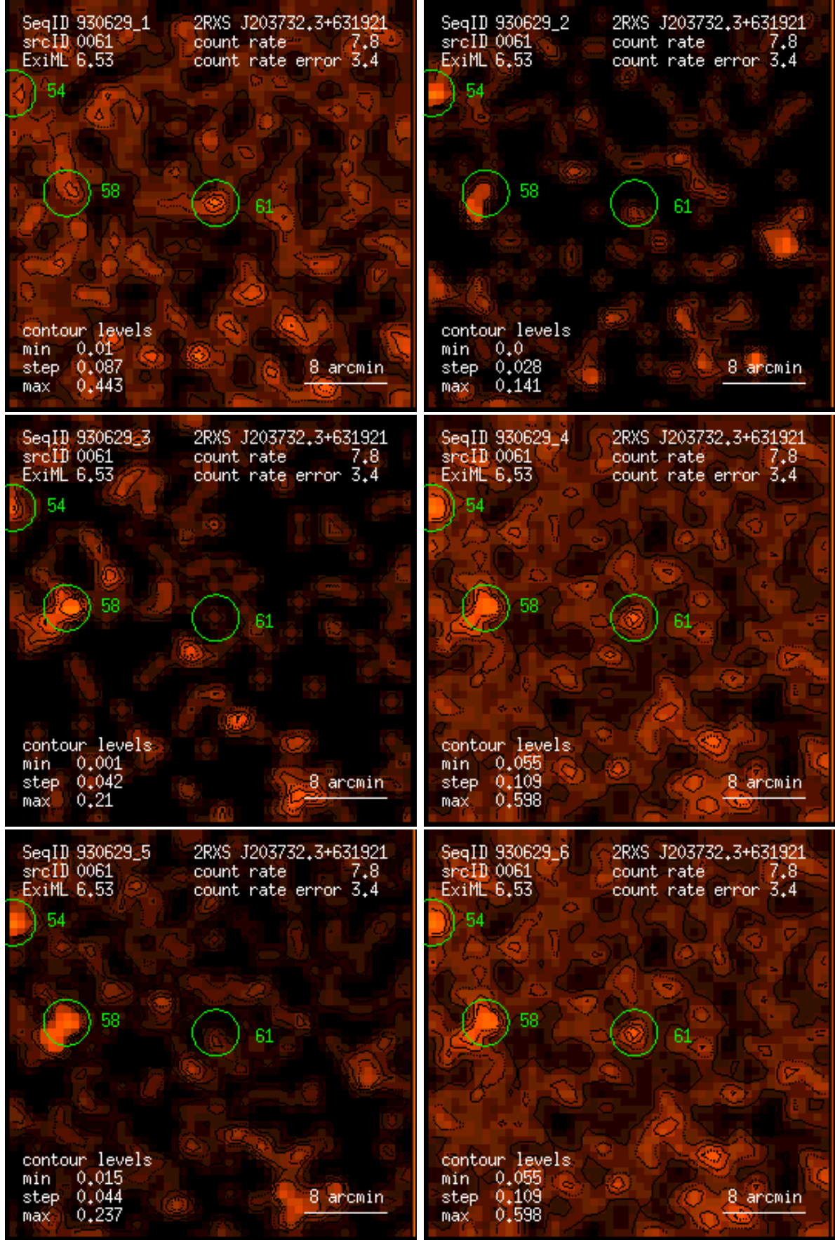
Figure 61: RASS 930629: detection 0061: band rate images, Gaussian filter: (1) PSPC channels 11 – 41, (2) 52 – 90, (3) 91 – 201, (4) 11 – 235, (5) 52 – 201, (6) 11 – 201. Broad band rates in counts/ks. Band rate contour levels in counts/ks/arcmin 2 .
