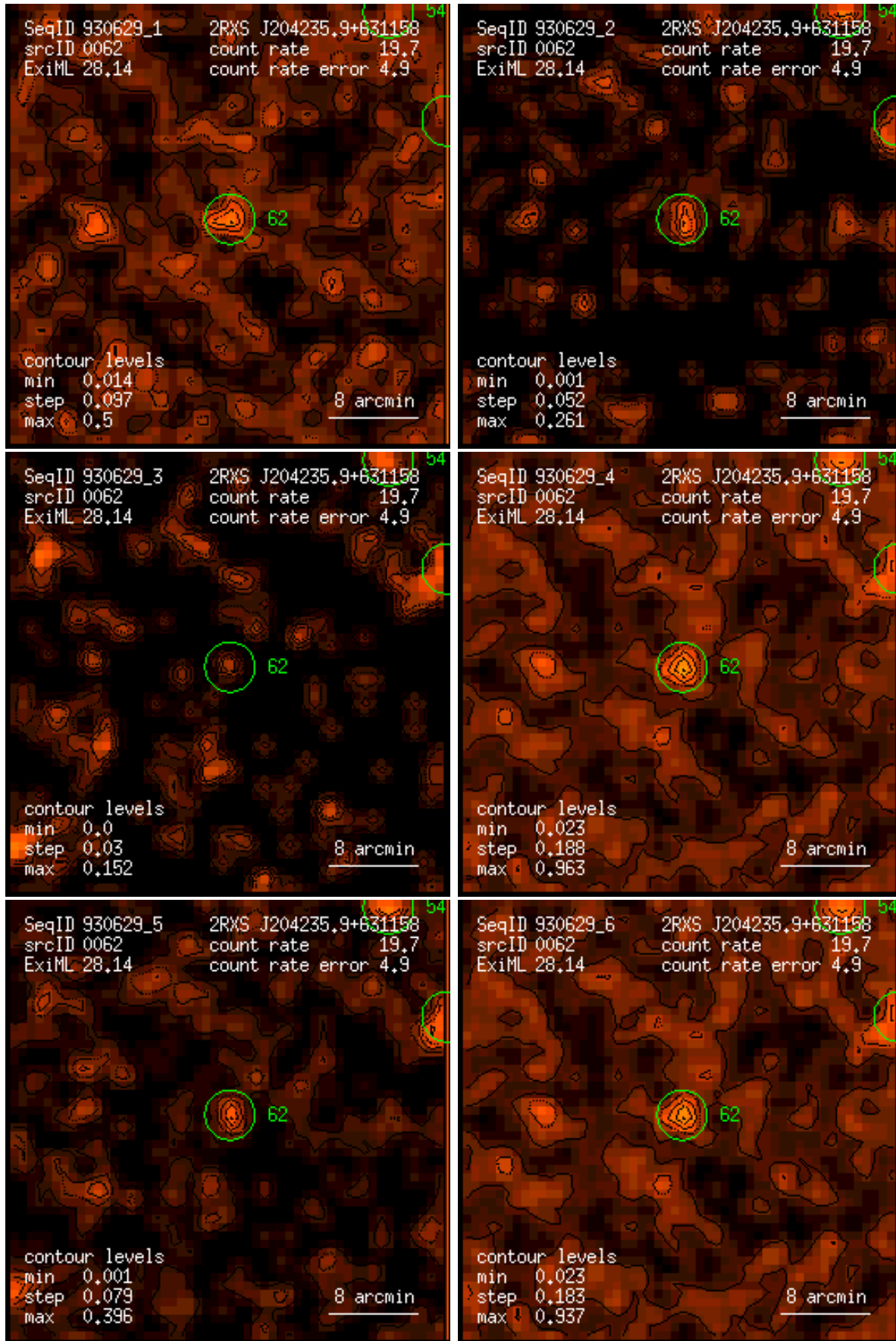
Figure 62: RASS 930629: detection 0062: band rate images, Gaussian filter: (1) PSPC channels 11 – 41, (2) 52 – 90, (3) 91 – 201, (4) 11 – 235, (5) 52 – 201, (6) 11 – 201. Broad band rates in counts/ks. Band rate contour levels in counts/ks/arcmin 2 .
