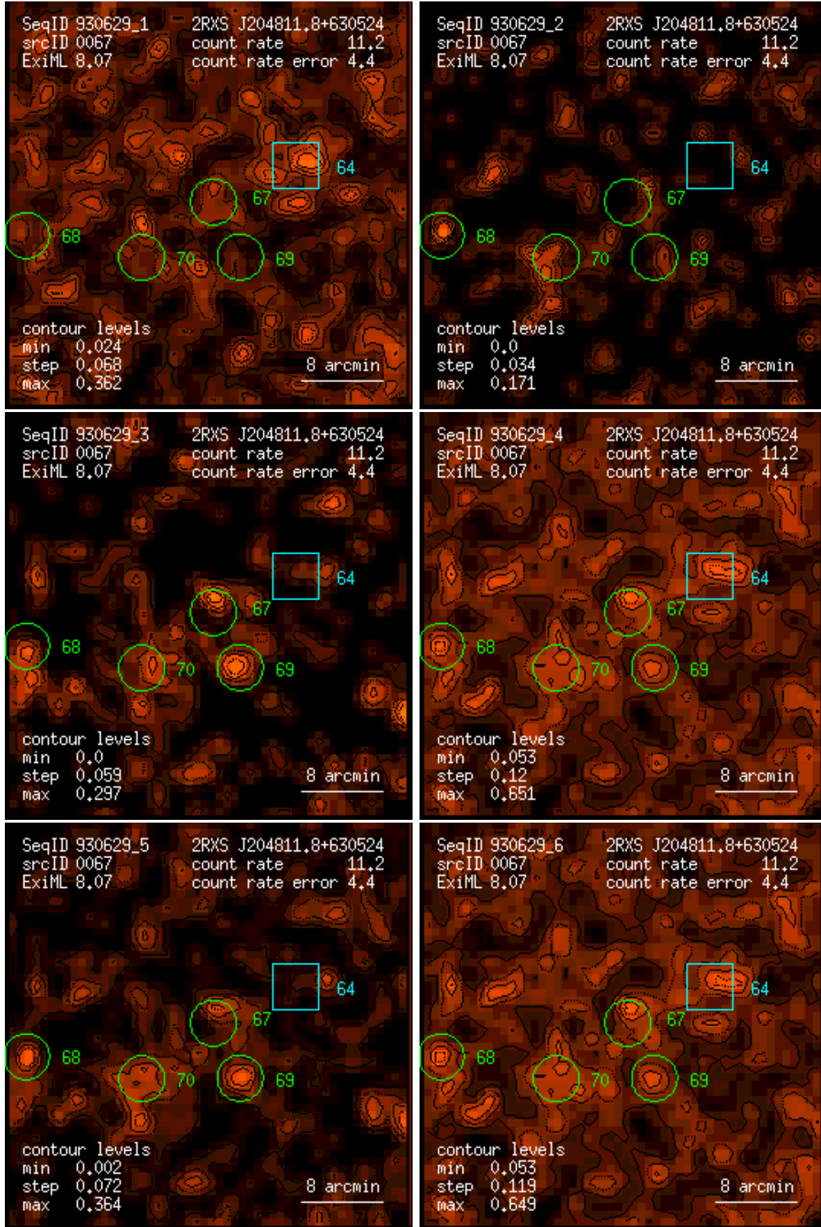
Figure 67: RASS 930629: detection 0067: band rate images, Gaussian filter: (1) PSPC channels 11 – 41, (2) 52 – 90, (3) 91 – 201, (4) 11 – 235, (5) 52 – 201, (6) 11 – 201. Broad band rates in counts/ks. Band rate contour levels in counts/ks/arcmin 2 .
