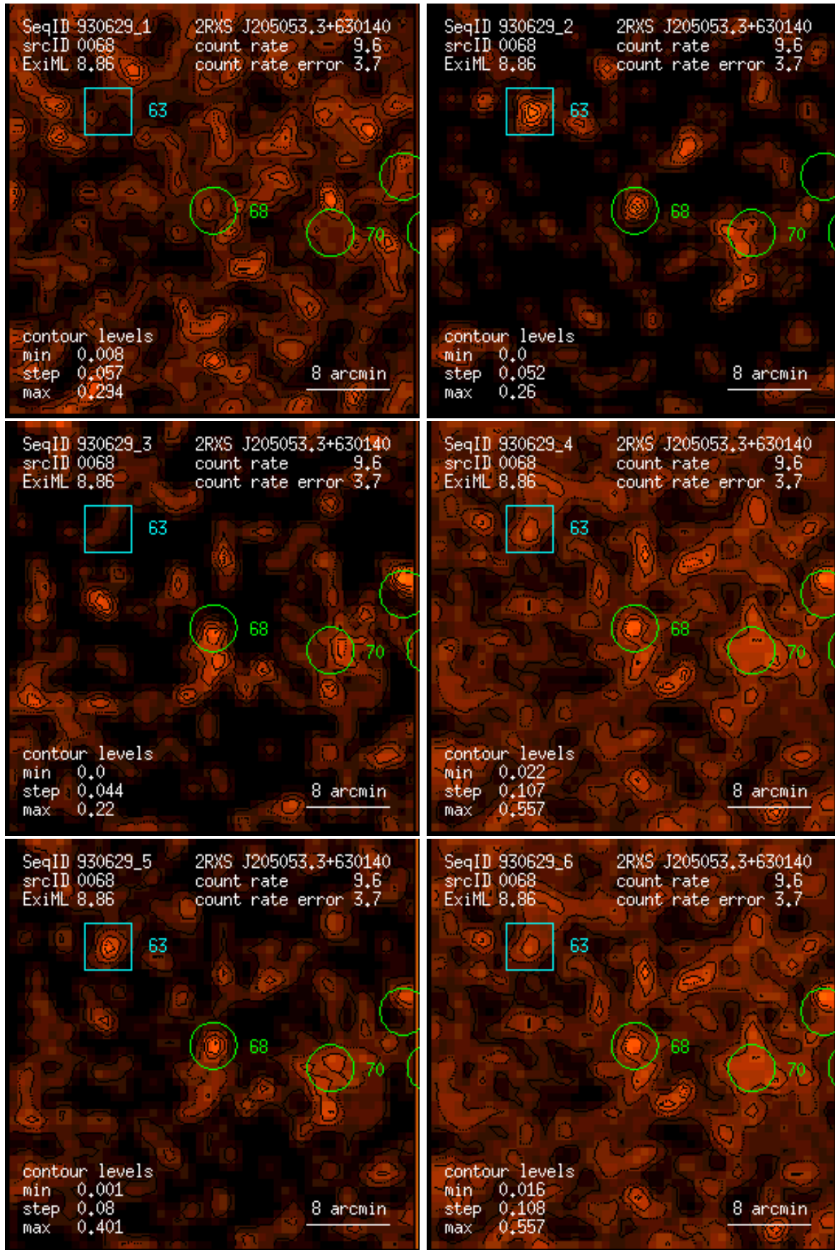
Figure 68: RASS 930629: detection 0068: band rate images, Gaussian filter: (1) PSPC channels 11 – 41, (2) 52 – 90, (3) 91 – 201, (4) 11 – 235, (5) 52 – 201, (6) 11 – 201. Broad band rates in counts/ks. Band rate contour levels in counts/ks/arcmin 2 .
