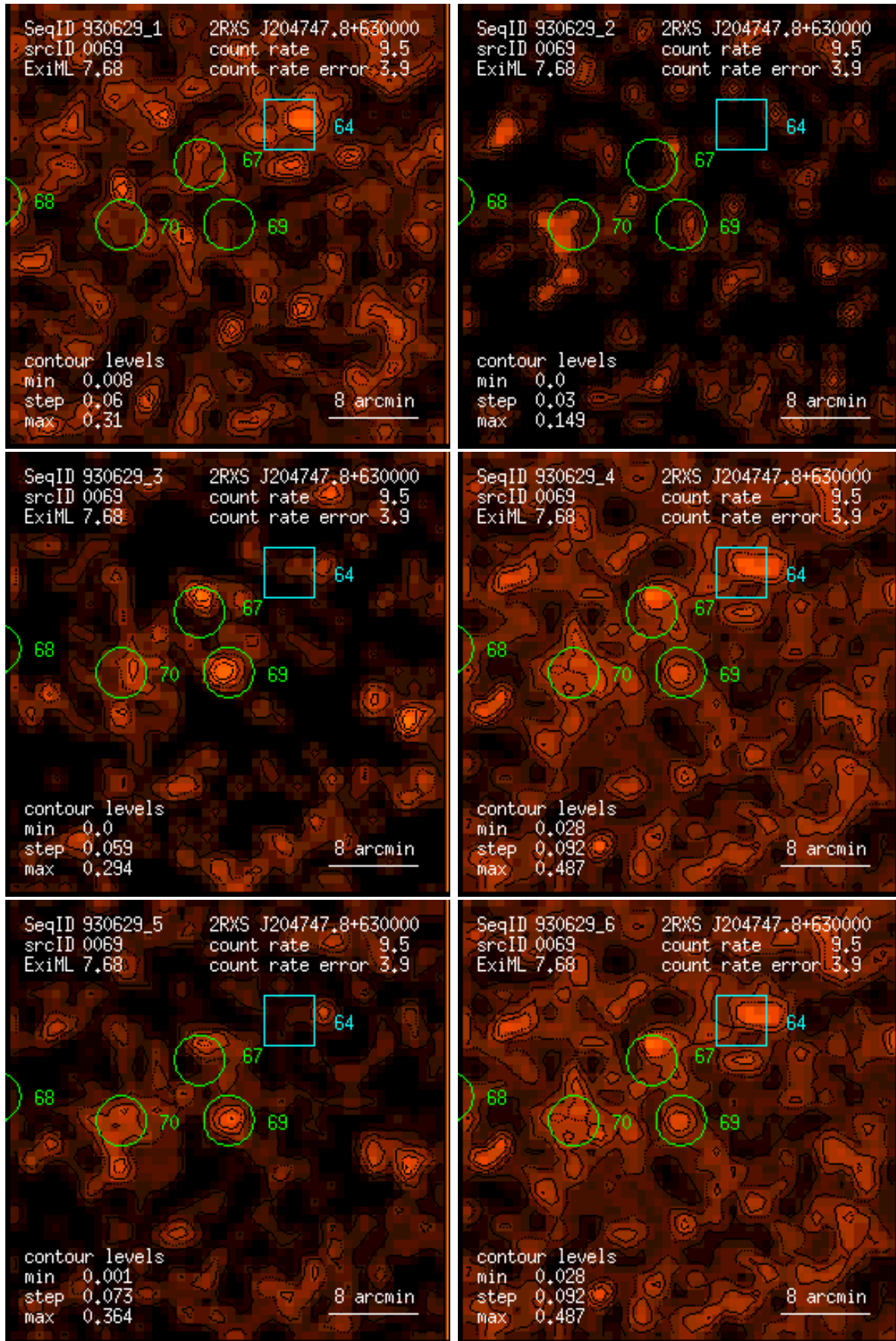
Figure 69: RASS 930629: detection 0069: band rate images, Gaussian filter: (1) PSPC channels 11 – 41, (2) 52 – 90, (3) 91 – 201, (4) 11 – 235, (5) 52 – 201, (6) 11 – 201. Broad band rates in counts/ks. Band rate contour levels in counts/ks/arcmin 2 .
