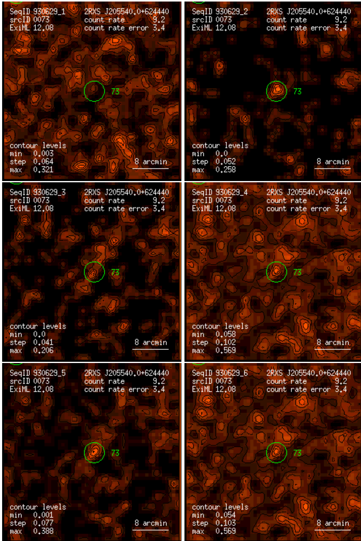
Figure 73: RASS 930629: detection 0073: band rate images, Gaussian filter: (1) PSPC channels 11 – 41, (2) 52 – 90, (3) 91 – 201, (4) 11 – 235, (5) 52 – 201, (6) 11 – 201. Broad band rates in counts/ks. Band rate contour levels in counts/ks/arcmin 2 .
