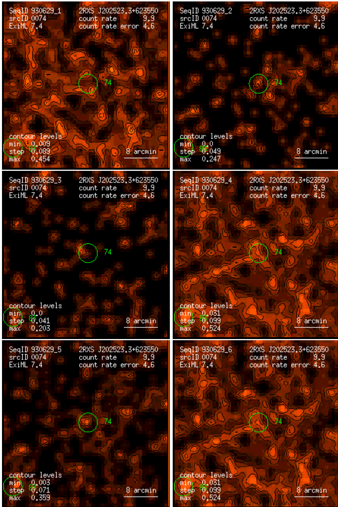
Figure 74: RASS 930629: detection 0074: band rate images, Gaussian filter: (1) PSPC channels 11 – 41, (2) 52 – 90, (3) 91 – 201, (4) 11 – 235, (5) 52 – 201, (6) 11 – 201. Broad band rates in counts/ks. Band rate contour levels in counts/ks/arcmin 2 .
