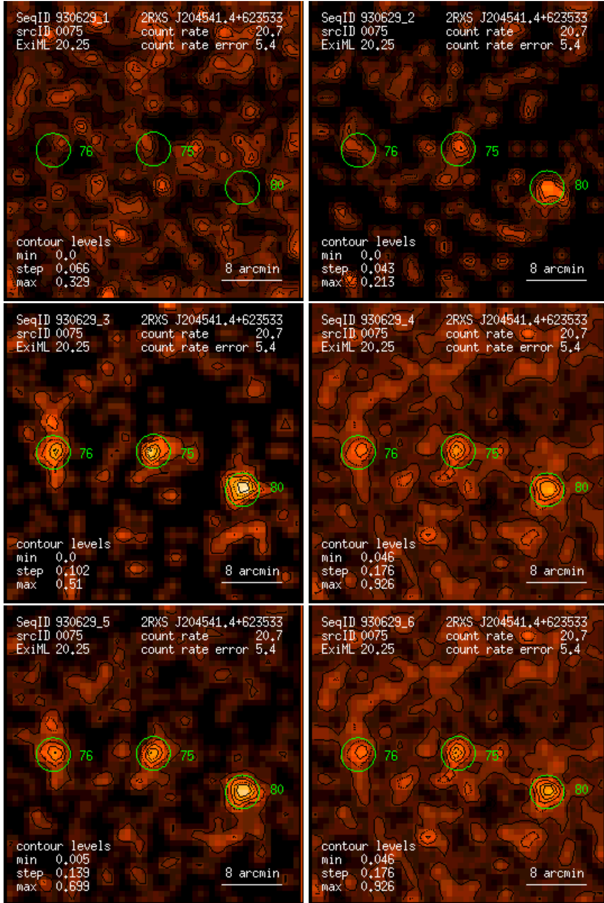
Figure 75: RASS 930629: detection 0075: band rate images, Gaussian filter: (1) PSPC channels 11 – 41, (2) 52 – 90, (3) 91 – 201, (4) 11 – 235, (5) 52 – 201, (6) 11 – 201. Broad band rates in counts/ks. Band rate contour levels in counts/ks/arcmin 2 .
