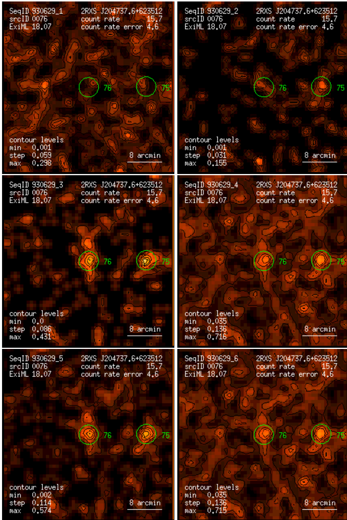
Figure 76: RASS 930629: detection 0076: band rate images, Gaussian filter: (1) PSPC channels 11 – 41, (2) 52 – 90, (3) 91 – 201, (4) 11 – 235, (5) 52 – 201, (6) 11 – 201. Broad band rates in counts/ks. Band rate contour levels in counts/ks/arcmin 2 .
