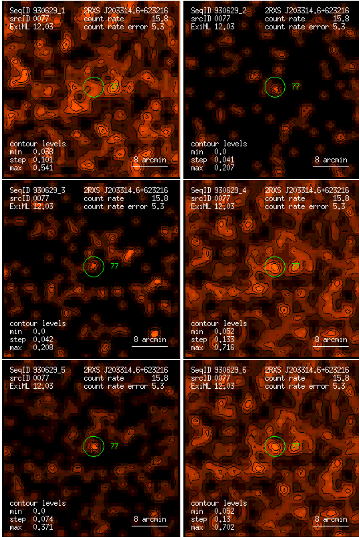
Figure 77: RASS 930629: detection 0077: band rate images, Gaussian filter: (1) PSPC channels 11 – 41, (2) 52 – 90, (3) 91 – 201, (4) 11 – 235, (5) 52 – 201, (6) 11 – 201. Broad band rates in counts/ks. Band rate contour levels in counts/ks/arcmin 2 .
