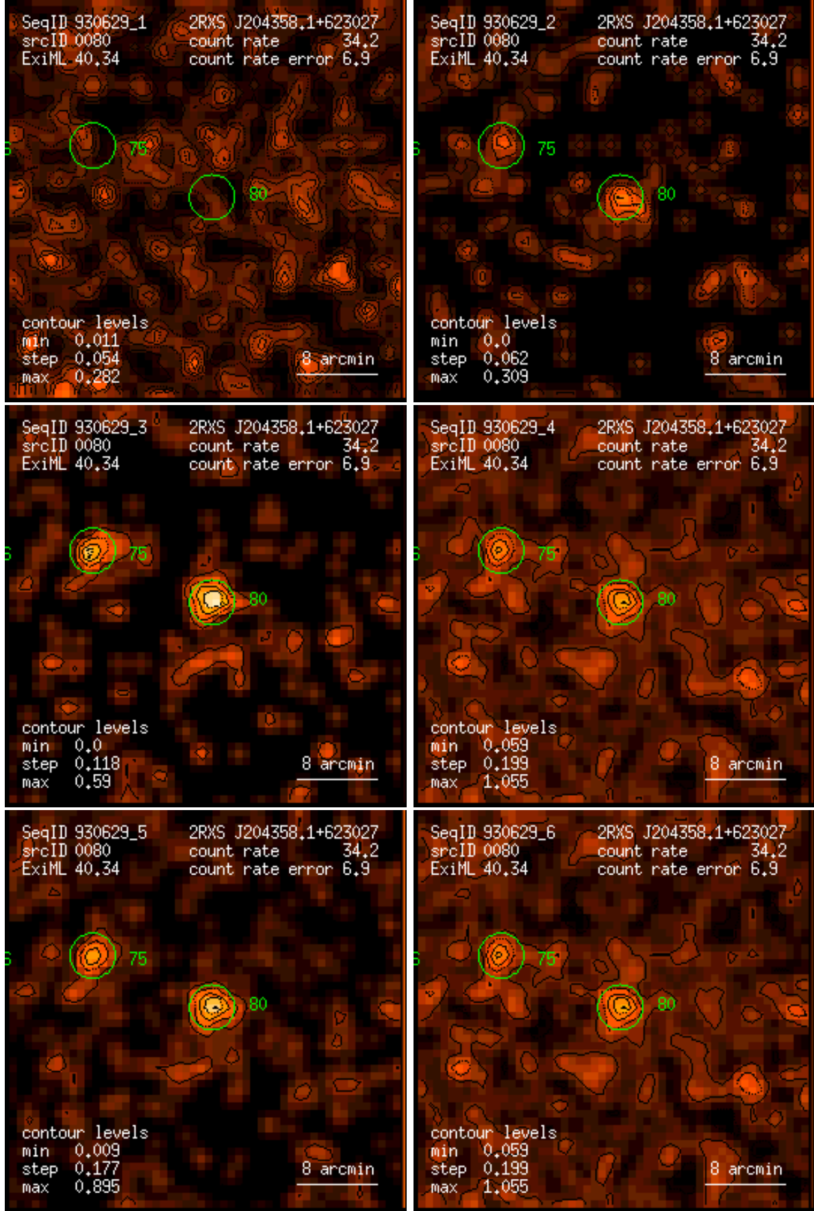
Figure 80: RASS 930629: detection 0080: band rate images, Gaussian filter: (1) PSPC channels 11 – 41, (2) 52 – 90, (3) 91 – 201, (4) 11 – 235, (5) 52 – 201, (6) 11 – 201. Broad band rates in counts/ks. Band rate contour levels in counts/ks/arcmin 2 .
