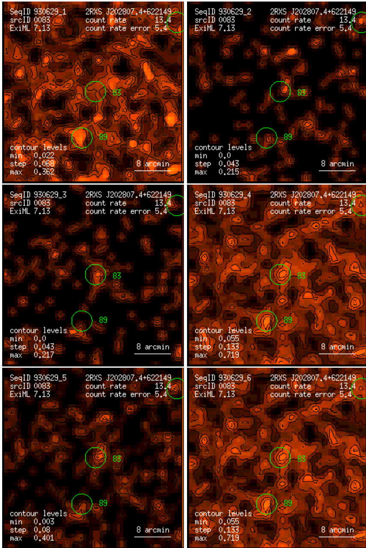
Figure 83: RASS 930629: detection 0083: band rate images, Gaussian filter: (1) PSPC channels 11 – 41, (2) 52 – 90, (3) 91 – 201, (4) 11 – 235, (5) 52 – 201, (6) 11 – 201. Broad band rates in counts/ks. Band rate contour levels in counts/ks/arcmin 2 .
