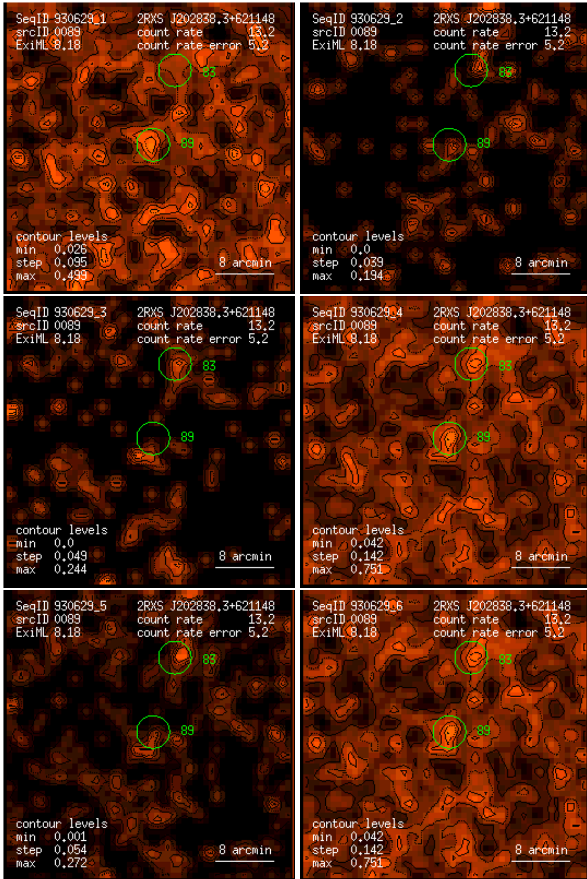
Figure 89: RASS 930629: detection 0089: band rate images, Gaussian filter: (1) PSPC channels 11 – 41, (2) 52 – 90, (3) 91 – 201, (4) 11 – 235, (5) 52 – 201, (6) 11 – 201. Broad band rates in counts/ks. Band rate contour levels in counts/ks/arcmin 2 .
