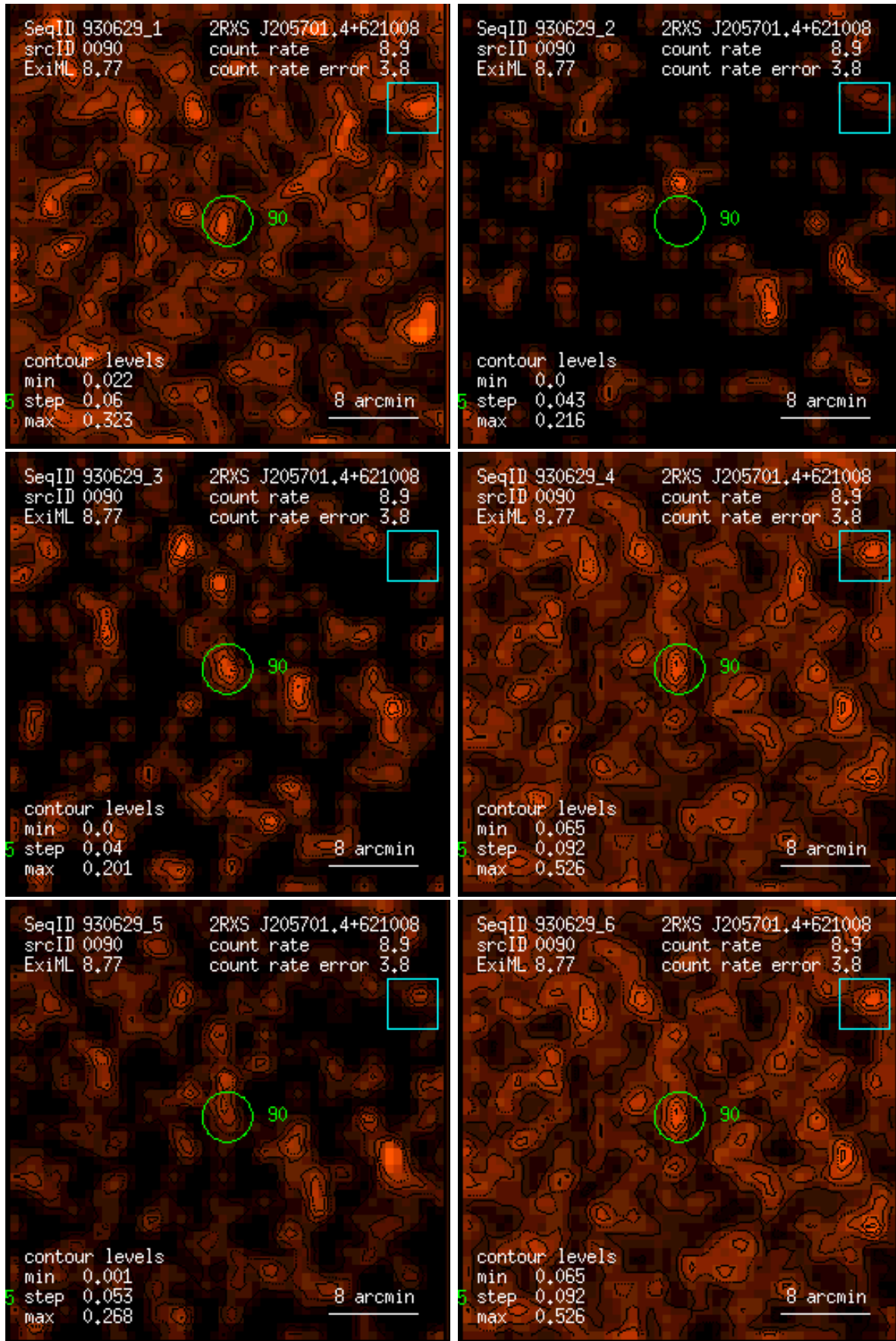
Figure 90: RASS 930629: detection 0090: band rate images, Gaussian filter: (1) PSPC channels 11 – 41, (2) 52 – 90, (3) 91 – 201, (4) 11 – 235, (5) 52 – 201, (6) 11 – 201. Broad band rates in counts/ks. Band rate contour levels in counts/ks/arcmin 2 .
