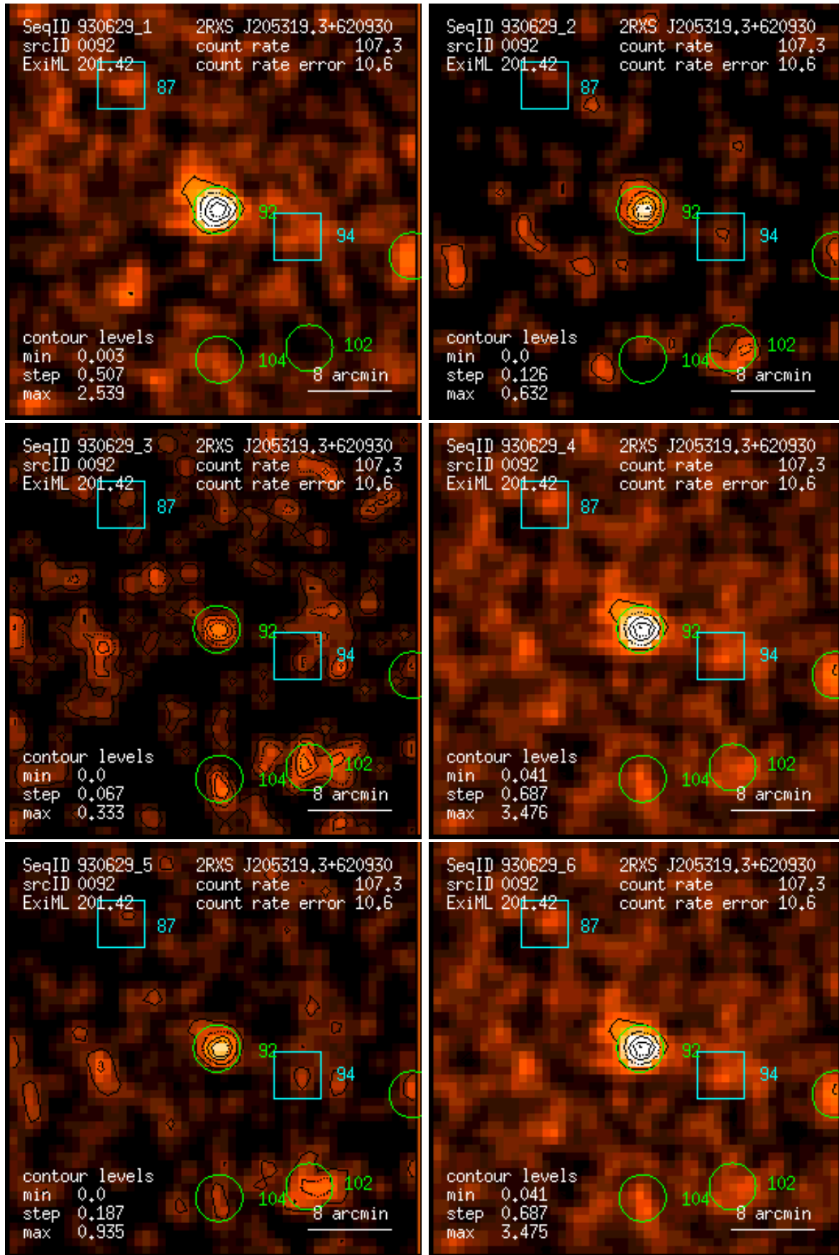
Figure 92: RASS 930629: detection 0092: band rate images, Gaussian filter: (1) PSPC channels 11 – 41, (2) 52 – 90, (3) 91 – 201, (4) 11 – 235, (5) 52 – 201, (6) 11 – 201. Broad band rates in counts/ks. Band rate contour levels in counts/ks/arcmin 2 .
