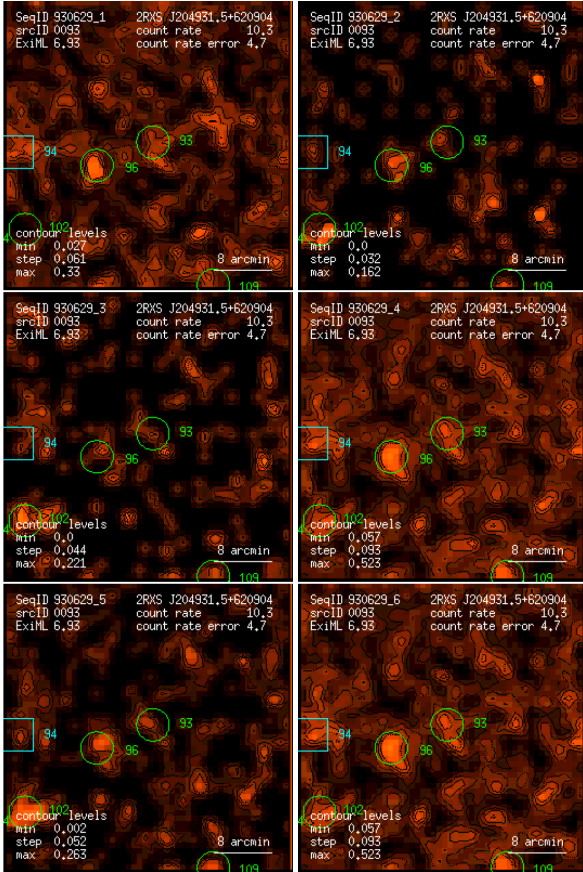
Figure 93: RASS 930629: detection 0093: band rate images, Gaussian filter: (1) PSPC channels 11 – 41, (2) 52 – 90, (3) 91 – 201, (4) 11 – 235, (5) 52 – 201, (6) 11 – 201. Broad band rates in counts/ks. Band rate contour levels in counts/ks/arcmin 2 .
