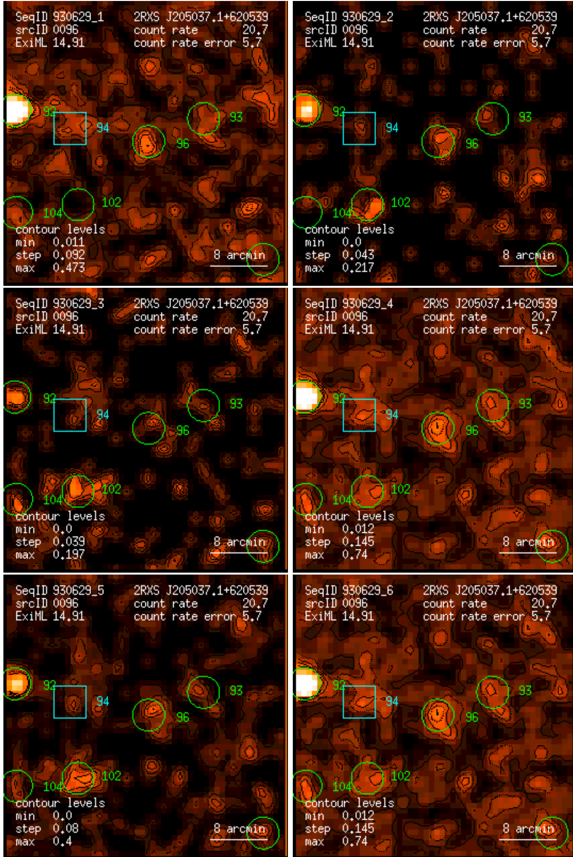
Figure 96: RASS 930629: detection 0096: band rate images, Gaussian filter: (1) PSPC channels 11 – 41, (2) 52 – 90, (3) 91 – 201, (4) 11 – 235, (5) 52 – 201, (6) 11 – 201. Broad band rates in counts/ks. Band rate contour levels in counts/ks/arcmin 2 .
