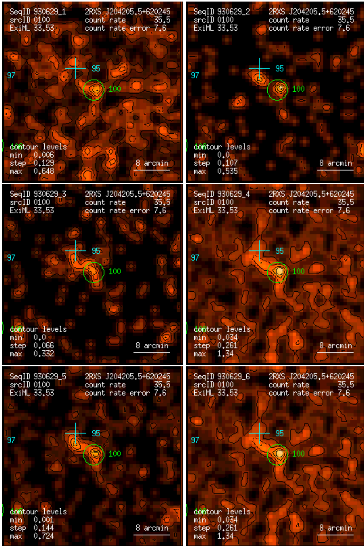
Figure 100: RASS 930629: detection 0100: band rate images, Gaussian filter: (1) PSPC channels 11 – 41, (2) 52 – 90, (3) 91 – 201, (4) 11 – 235, (5) 52 – 201, (6) 11 – 201. Broad band rates in counts/ks. Band rate contour levels in counts/ks/arcmin 2 .
