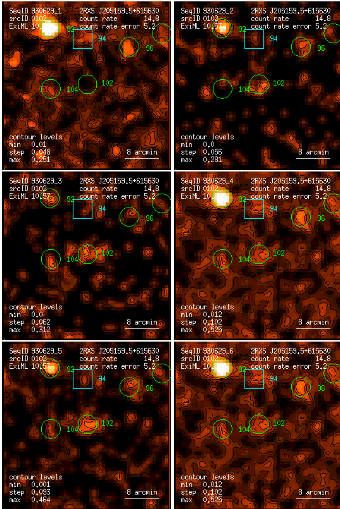
Figure 102: RASS 930629: detection 0102: band rate images, Gaussian filter: (1) PSPC channels 11 – 41, (2) 52 – 90, (3) 91 – 201, (4) 11 – 235, (5) 52 – 201, (6) 11 – 201. Broad band rates in counts/ks. Band rate contour levels in counts/ks/arcmin 2 .
