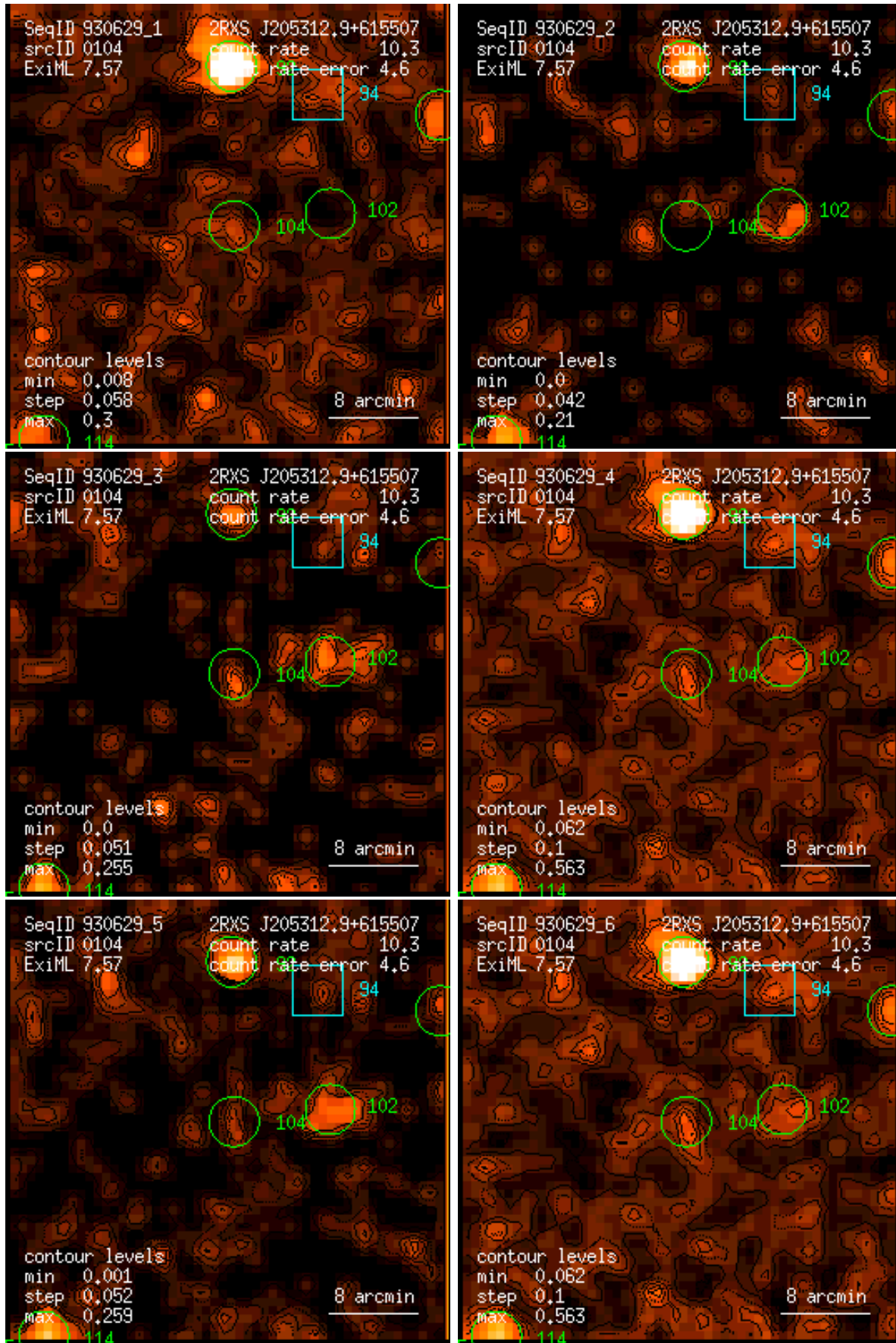
Figure 104: RASS 930629: detection 0104: band rate images, Gaussian filter: (1) PSPC channels 11 – 41, (2) 52 – 90, (3) 91 – 201, (4) 11 – 235, (5) 52 – 201, (6) 11 – 201. Broad band rates in counts/ks. Band rate contour levels in counts/ks/arcmin 2 .
