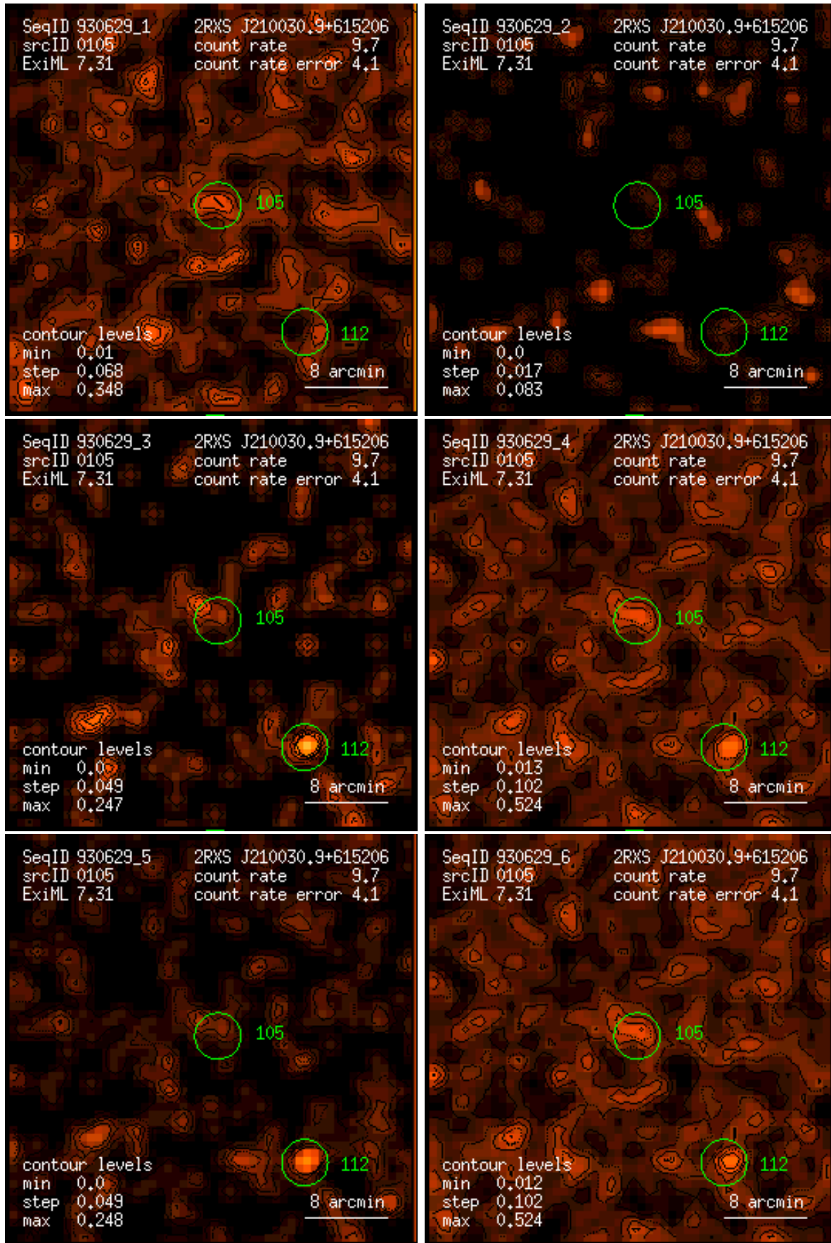
Figure 105: RASS 930629: detection 0105: band rate images, Gaussian filter: (1) PSPC channels 11 – 41, (2) 52 – 90, (3) 91 – 201, (4) 11 – 235, (5) 52 – 201, (6) 11 – 201. Broad band rates in counts/ks. Band rate contour levels in counts/ks/arcmin 2 .
