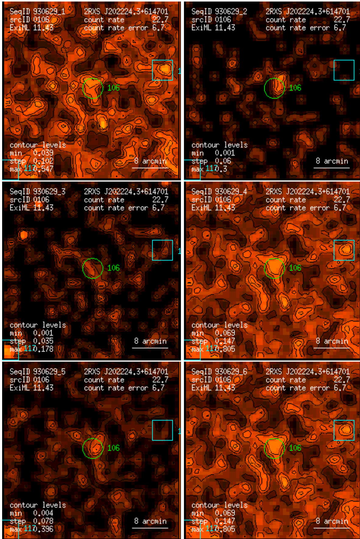
Figure 106: RASS 930629: detection 0106: band rate images, Gaussian filter: (1) PSPC channels 11 – 41, (2) 52 – 90, (3) 91 – 201, (4) 11 – 235, (5) 52 – 201, (6) 11 – 201. Broad band rates in counts/ks. Band rate contour levels in counts/ks/arcmin 2 .
