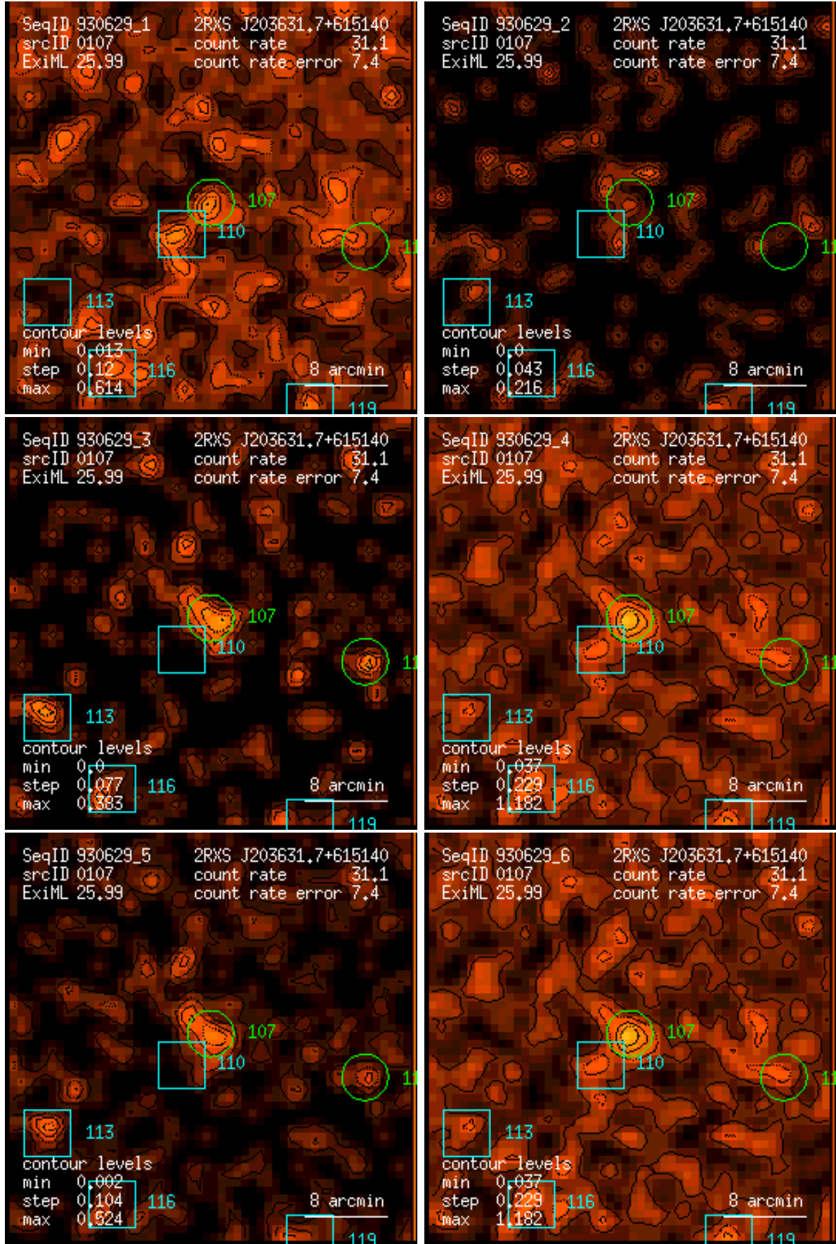
Figure 107: RASS 930629: detection 0107: band rate images, Gaussian filter: (1) PSPPC channels 11 – 41, (2) 52 – 90, (3) 91 – 201, (4) 11 – 235, (5) 52 – 201, (6) 11 – 201. Broad band rates in counts/ks. Band rate contour levels in counts/ks/arcmin 2 .
