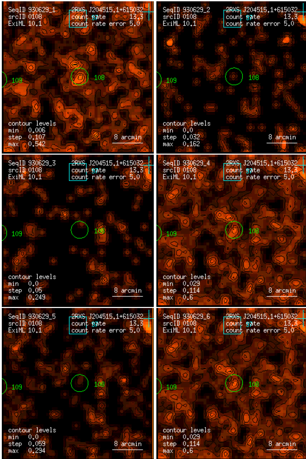
Figure 108: RASS 930629: detection 0108: band rate images, Gaussian filter: (1) PSPC channels 11 – 41, (2) 52 – 90, (3) 91 – 201, (4) 11 – 235, (5) 52 – 201, (6) 11 – 201. Broad band rates in counts/ks. Band rate contour levels in counts/ks/arcmin 2 .
