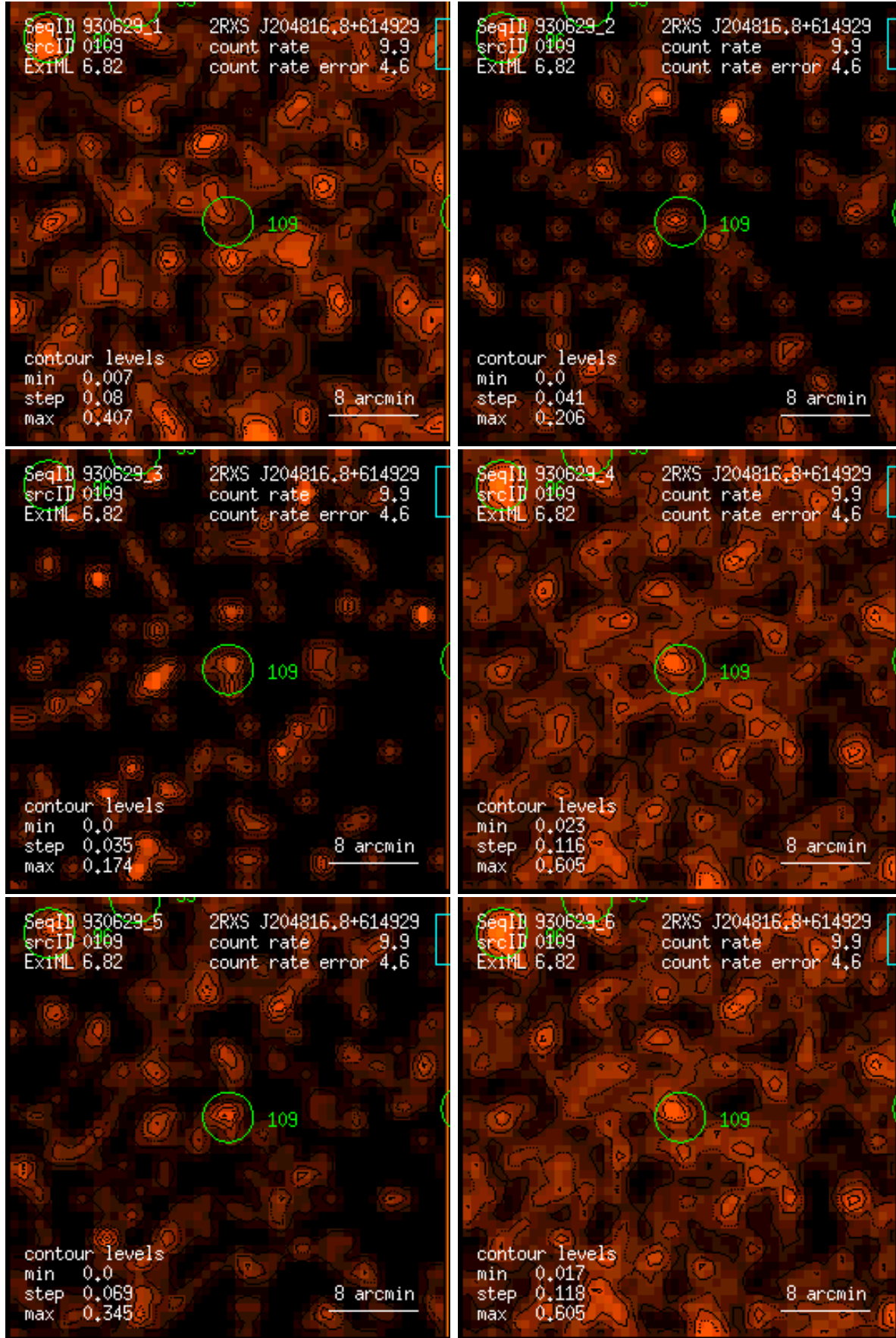
Figure 109: RASS 930629: detection 0109: band rate images, Gaussian filter: (1) PSPC channels 11 – 41, (2) 52 – 90, (3) 91 – 201, (4) 11 – 235, (5) 52 – 201, (6) 11 – 201. Broad band rates in counts/ks. Band rate contour levels in counts/ks/arcmin 2 .
