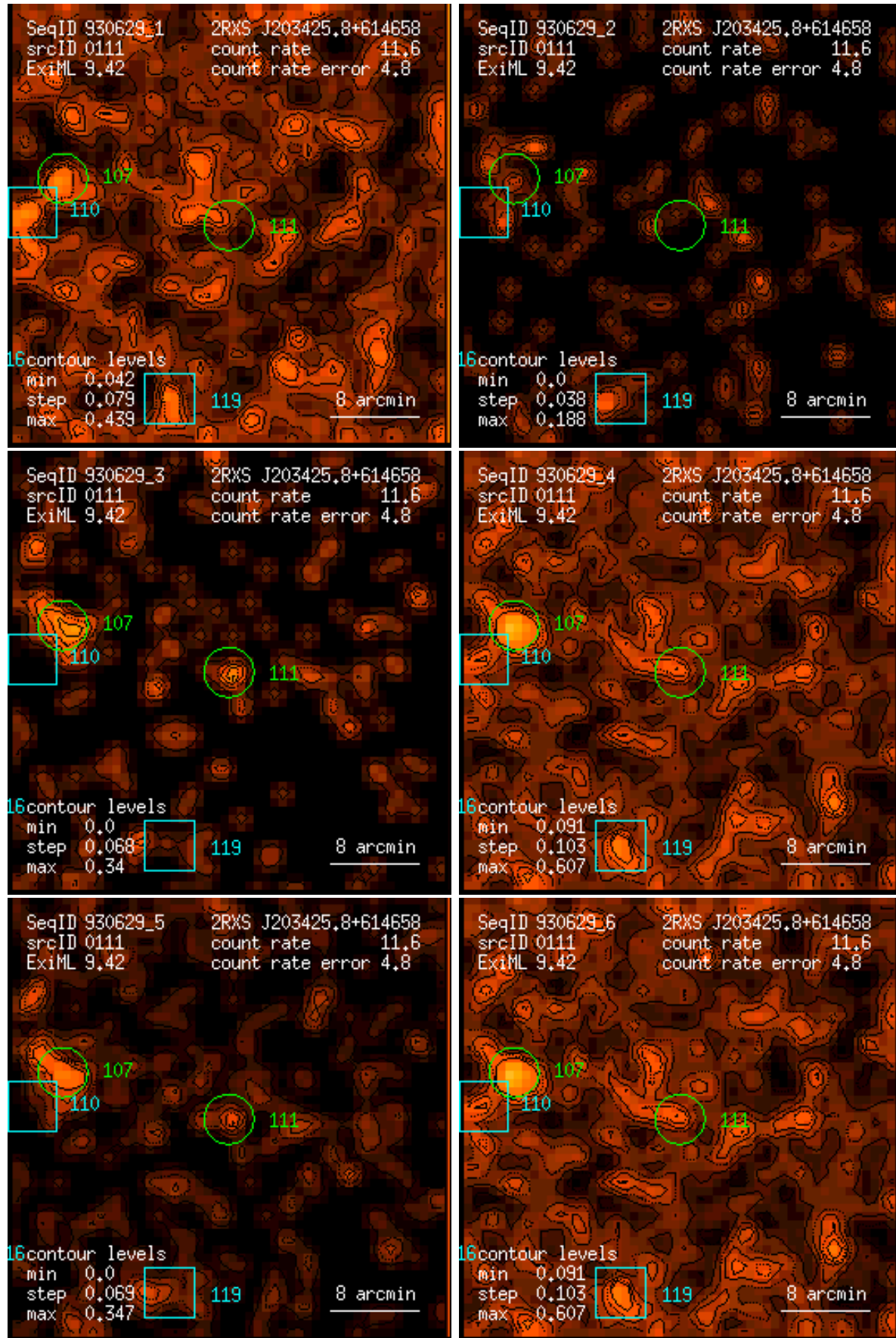
Figure 111: RASS 930629: detection 0111: band rate images, Gaussian filter: (1) PSPC channels 11 – 41, (2) 52 – 90, (3) 91 – 201, (4) 11 – 235, (5) 52 – 201, (6) 11 – 201. Broad band rates in counts/ks. Band rate contour levels in counts/ks/arcmin 2 .
