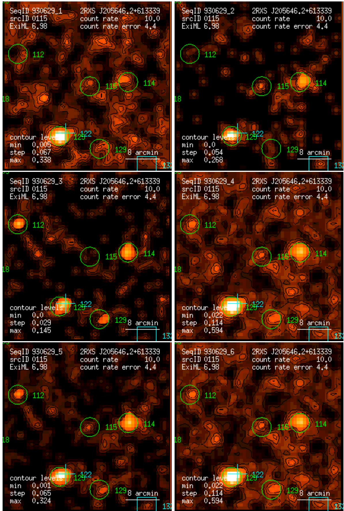
Figure 115: RASS 930629: detection 0115: band rate images, Gaussian filter: (1) PSPC channels 11 – 41, (2) 52 – 90, (3) 91 – 201, (4) 11 – 235, (5) 52 – 201, (6) 11 – 201. Broad band rates in counts/ks. Band rate contour levels in counts/ks/arcmin 2 .
