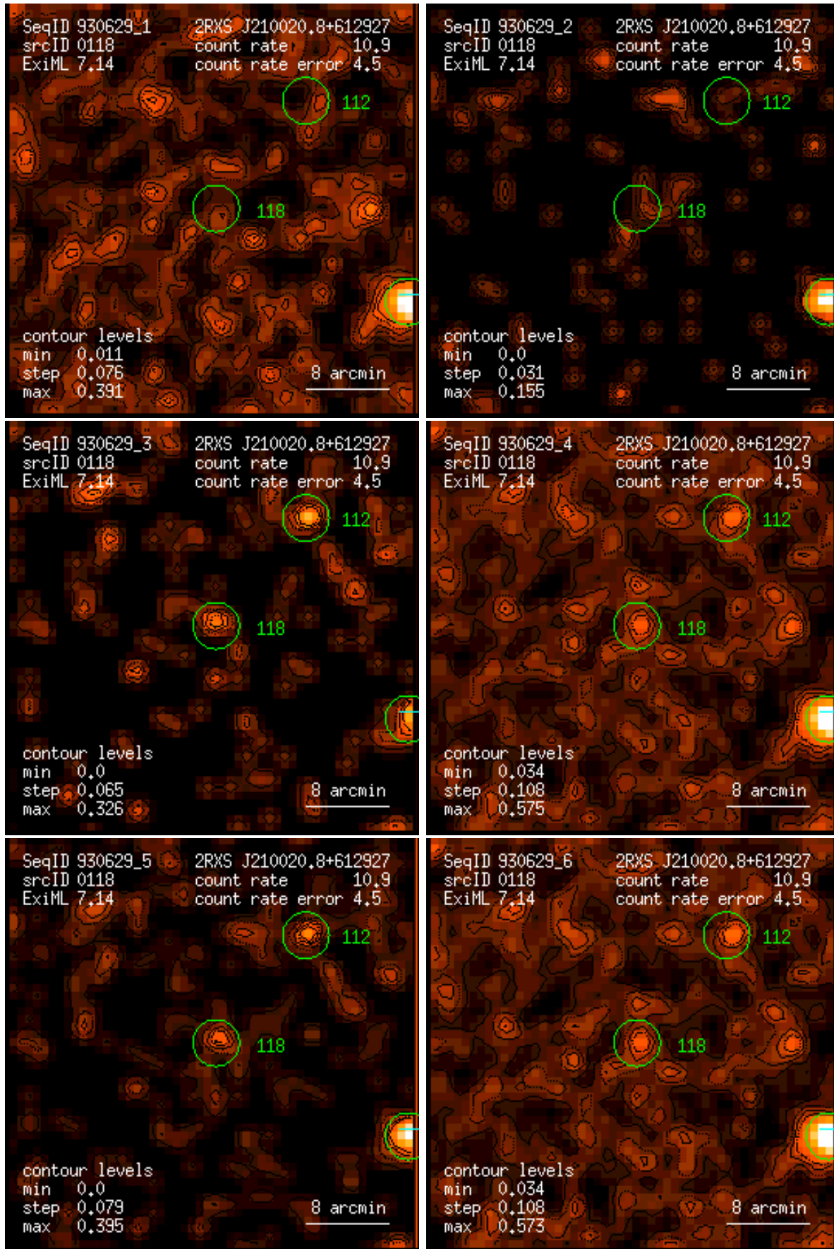
Figure 118: RASS 930629: detection 0118: band rate images, Gaussian filter: (1) PSPC channels 11 – 41, (2) 52 – 90, (3) 91 – 201, (4) 11 – 235, (5) 52 – 201, (6) 11 – 201. Broad band rates in counts/ks. Band rate contour levels in counts/ks/arcmin 2 .
