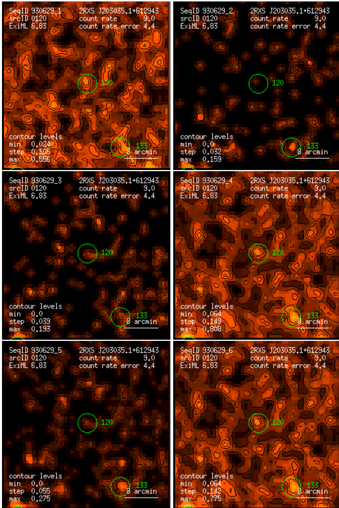
Figure 120: RASS 930629: detection 0120: band rate images, Gaussian filter: (1) PSPC channels 11 – 41, (2) 52 – 90, (3) 91 – 201, (4) 11 – 235, (5) 52 – 201, (6) 11 – 201. Broad band rates in counts/ks. Band rate contour levels in counts/ks/arcmin 2 .
