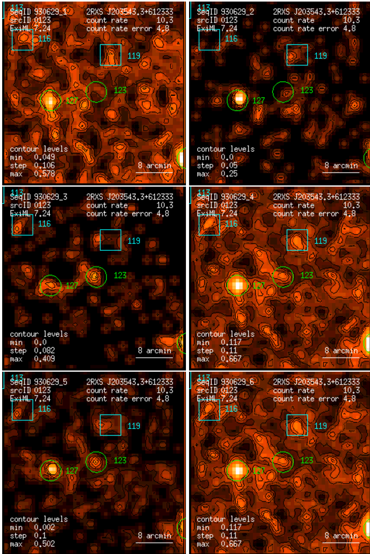
Figure 123: RASS 930629: detection 0123: band rate images, Gaussian filter: (1) PSPC channels 11 – 41, (2) 52 – 90, (3) 91 – 201, (4) 11 – 235, (5) 52 – 201, (6) 11 – 201. Broad band rates in counts/ks. Band rate contour levels in counts/ks/arcmin 2 .
