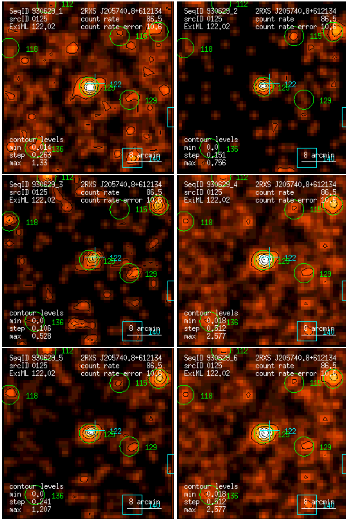
Figure 125: RASS 930629: detection 0125: band rate images, Gaussian filter: (1) PSPC channels 11 – 41, (2) 52 – 90, (3) 91 – 201, (4) 11 – 235, (5) 52 – 201, (6) 11 – 201. Broad band rates in counts/ks. Band rate contour levels in counts/ks/arcmin 2 .
