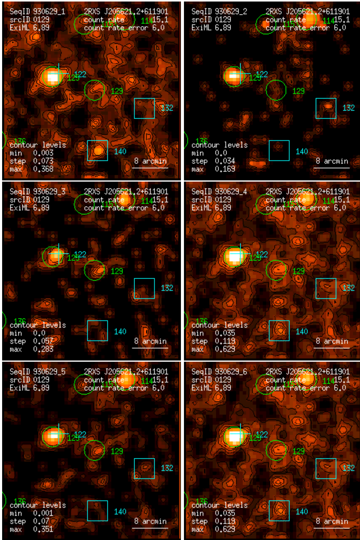
Figure 129: RASS 930629: detection 0129: band rate images, Gaussian filter: (1) PSPC channels 11 – 41, (2) 52 – 90, (3) 91 – 201, (4) 11 – 235, (5) 52 – 201, (6) 11 – 201. Broad band rates in counts/ks. Band rate contour levels in counts/ks/arcmin 2 .
