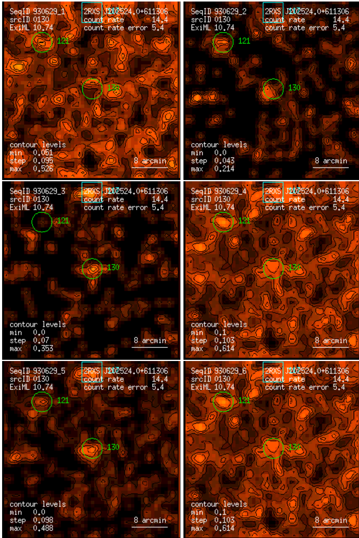
Figure 130: RASS 930629: detection 0130: band rate images, Gaussian filter: (1) PSPC channels 11 – 41, (2) 52 – 90, (3) 91 – 201, (4) 11 – 235, (5) 52 – 201, (6) 11 – 201. Broad band rates in counts/ks. Band rate contour levels in counts/ks/arcmin 2 .
