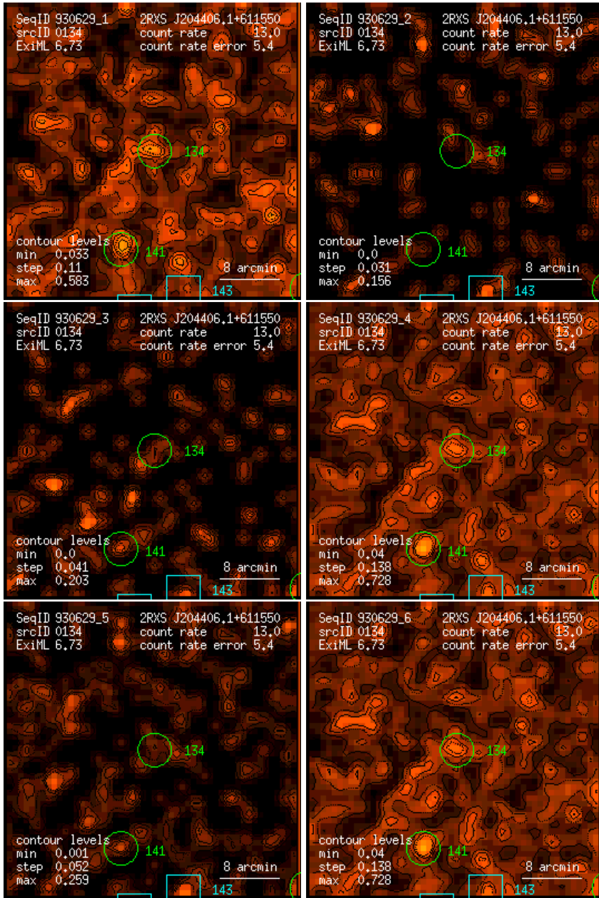
Figure 134: RASS 930629: detection 0134: band rate images, Gaussian filter: (1) PSPC channels 11 – 41, (2) 52 – 90, (3) 91 – 201, (4) 11 – 235, (5) 52 – 201, (6) 11 – 201. Broad band rates in counts/ks. Band rate contour levels in counts/ks/arcmin 2 .
