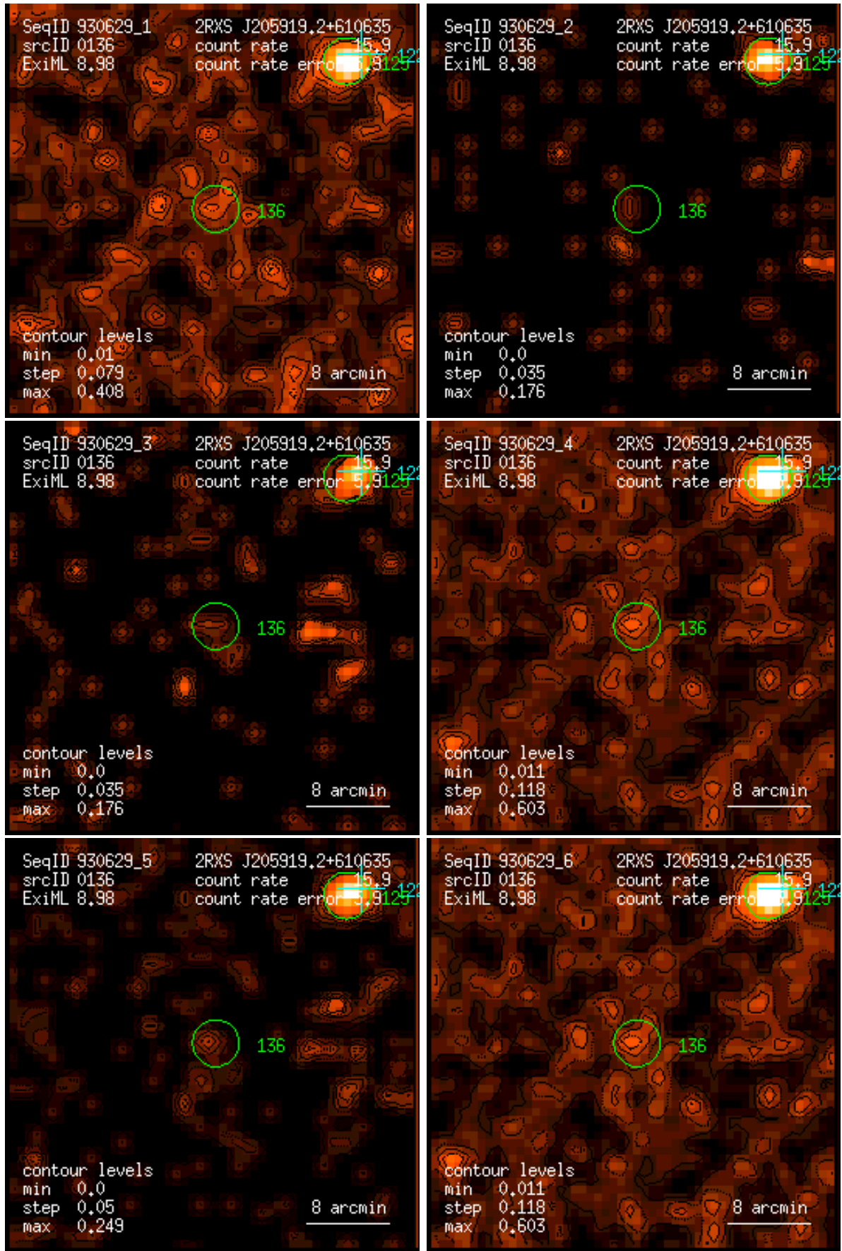
Figure 136: RASS 930629: detection 0136: band rate images, Gaussian filter: (1) PSPC channels 11 – 41, (2) 52 – 90, (3) 91 – 201, (4) 11 – 235, (5) 52 – 201, (6) 11 – 201. Broad band rates in counts/ks. Band rate contour levels in counts/ks/arcmin 2 .
