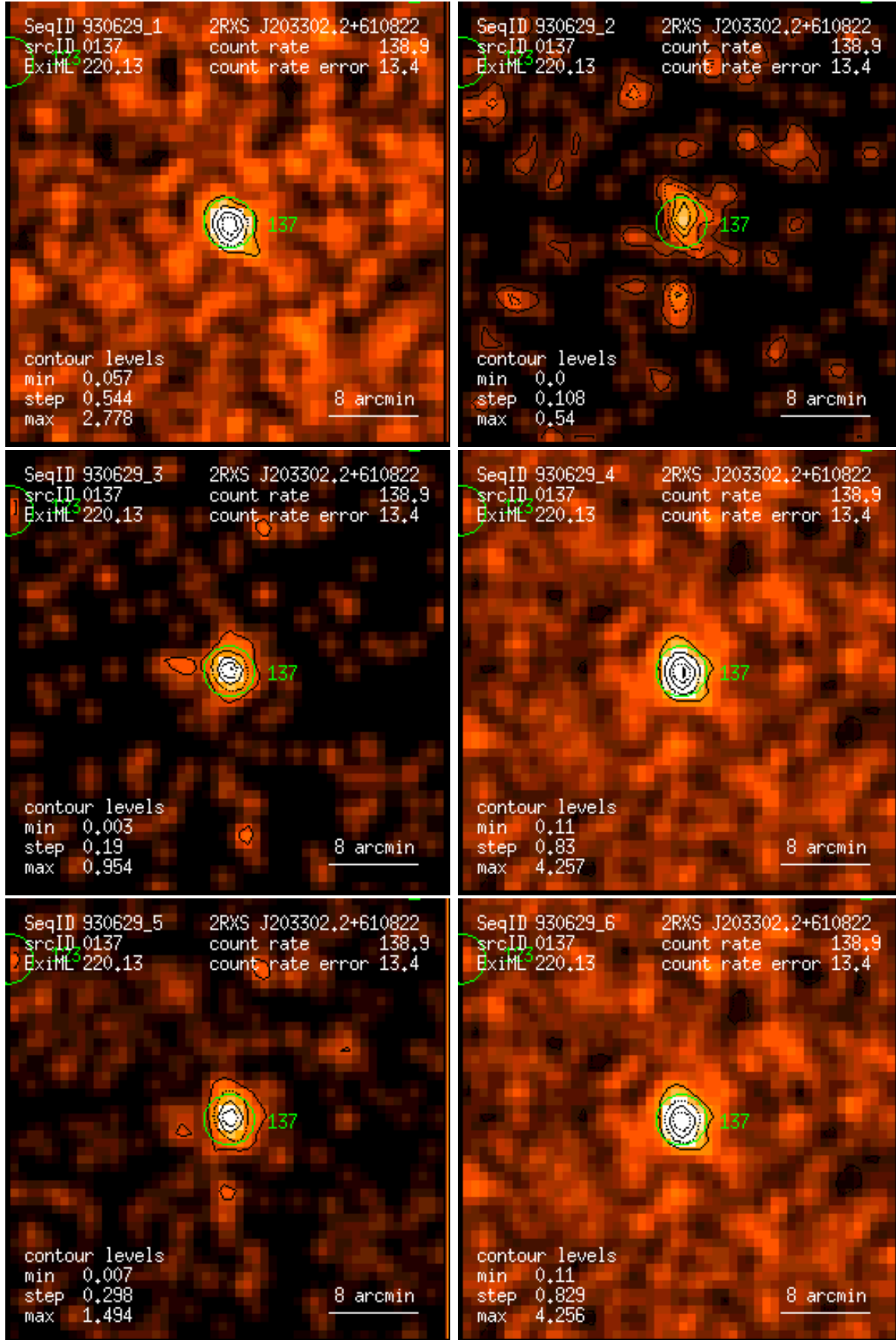
Figure 137: RASS 930629: detection 0137: band rate images, Gaussian filter: (1) PSPC channels 11 – 41, (2) 52 – 90, (3) 91 – 201, (4) 11 – 235, (5) 52 – 201, (6) 11 – 201. Broad band rates in counts/ks. Band rate contour levels in counts/ks/arcmin 2 .
