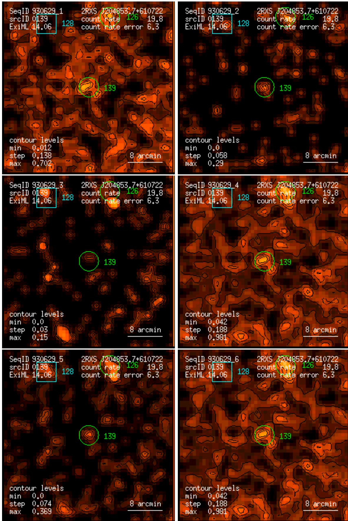
Figure 139: RASS 930629: detection 0139: band rate images, Gaussian filter: (1) PSPC channels 11 – 41, (2) 52 – 90, (3) 91 – 201, (4) 11 – 235, (5) 52 – 201, (6) 11 – 201. Broad band rates in counts/ks. Band rate contour levels in counts/ks/arcmin 2 .
