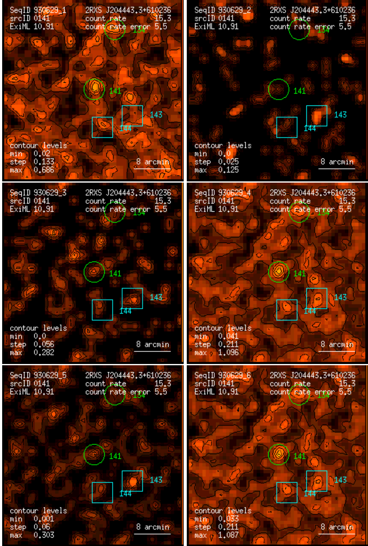
Figure 141: RASS 930629: detection 0141: band rate images, Gaussian filter: (1) PSPC channels 11 – 41, (2) 52 – 90, (3) 91 – 201, (4) 11 – 235, (5) 52 – 201, (6) 11 – 201. Broad band rates in counts/ks. Band rate contour levels in counts/ks/arcmin 2 .
