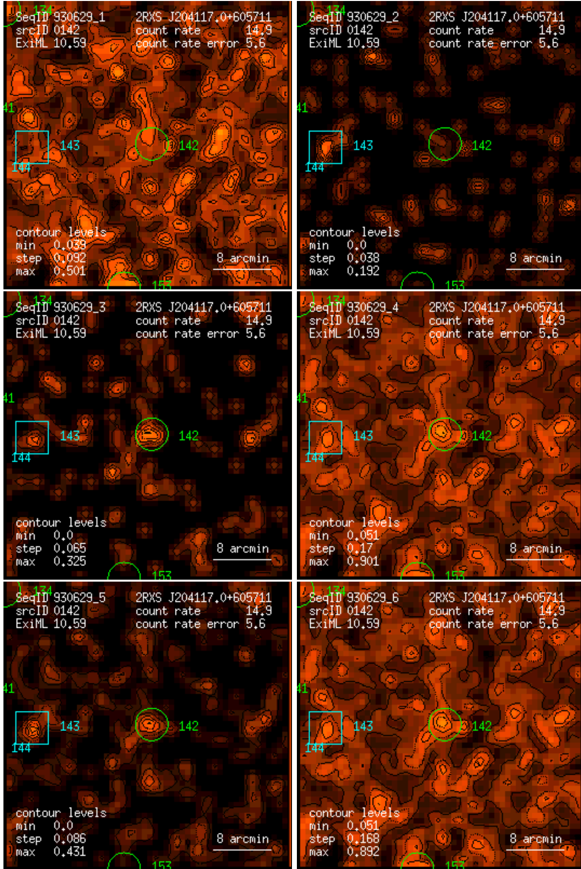
Figure 142: RASS 930629: detection 0142: band rate images, Gaussian filter: (1) PSPC channels 11 – 41, (2) 52 – 90, (3) 91 – 201, (4) 11 – 235, (5) 52 – 201, (6) 11 – 201. Broad band rates in counts/ks. Band rate contour levels in counts/ks/arcmin 2 .
