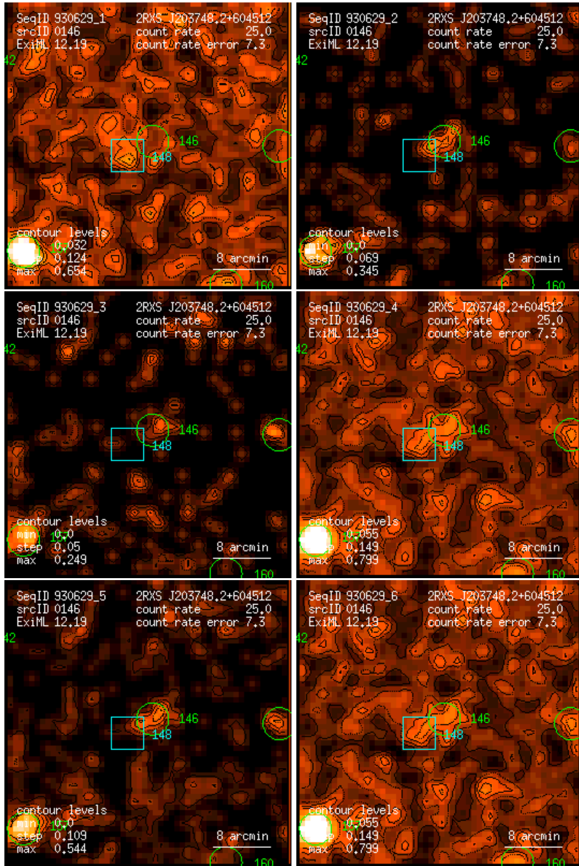
Figure 146: RASS 930629: detection 0146: band rate images, Gaussian filter: (1) PSPC channels 11 – 41, (2) 52 – 90, (3) 91 – 201, (4) 11 – 235, (5) 52 – 201, (6) 11 – 201. Broad band rates in counts/ks. Band rate contour levels in counts/ks/arcmin 2 .
