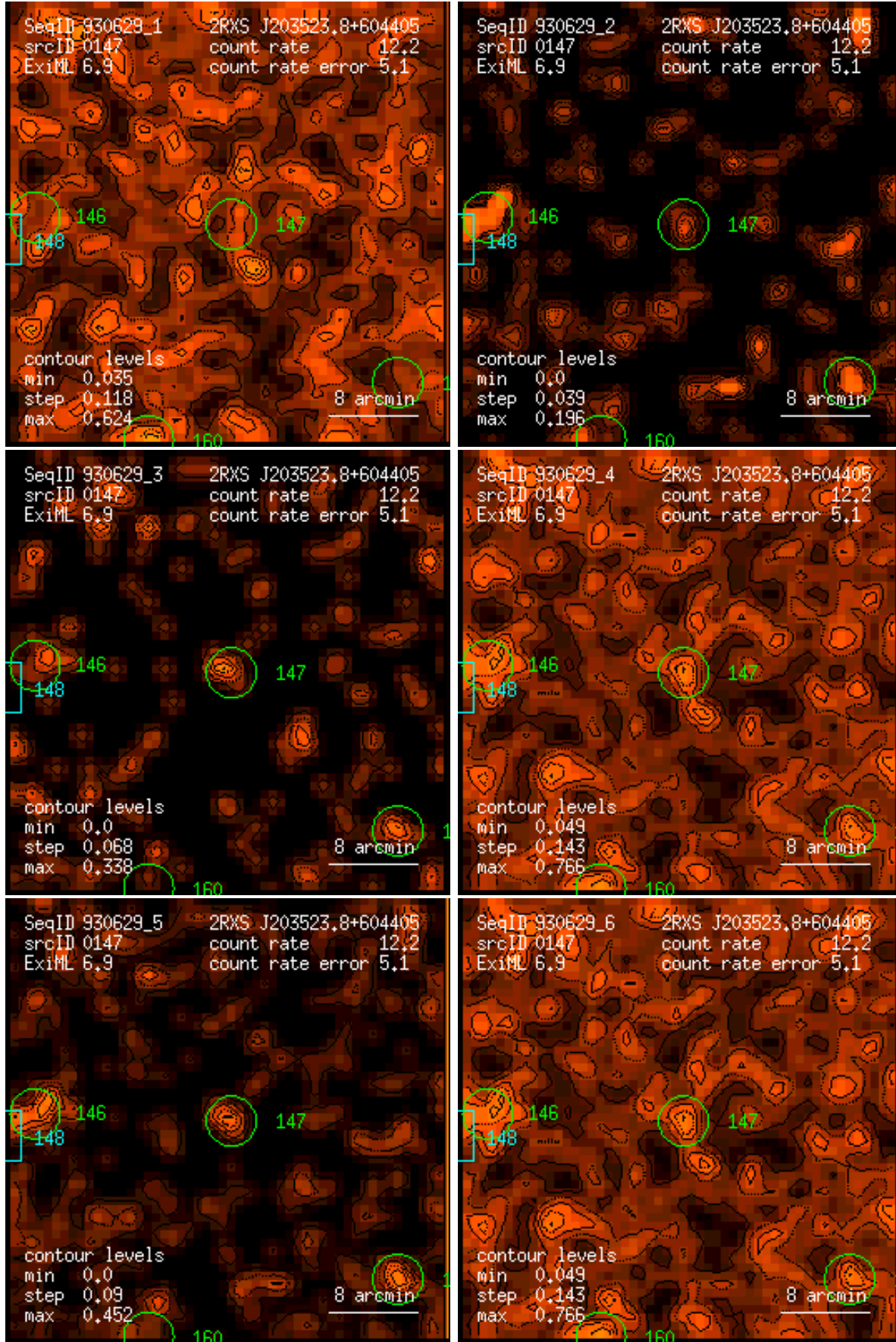
Figure 147: RASS 930629: detection 0147: band rate images, Gaussian filter: (1) PSPC channels 11 – 41, (2) 52 – 90, (3) 91 – 201, (4) 11 – 235, (5) 52 – 201, (6) 11 – 201. Broad band rates in counts/ks. Band rate contour levels in counts/ks/arcmin 2 .
