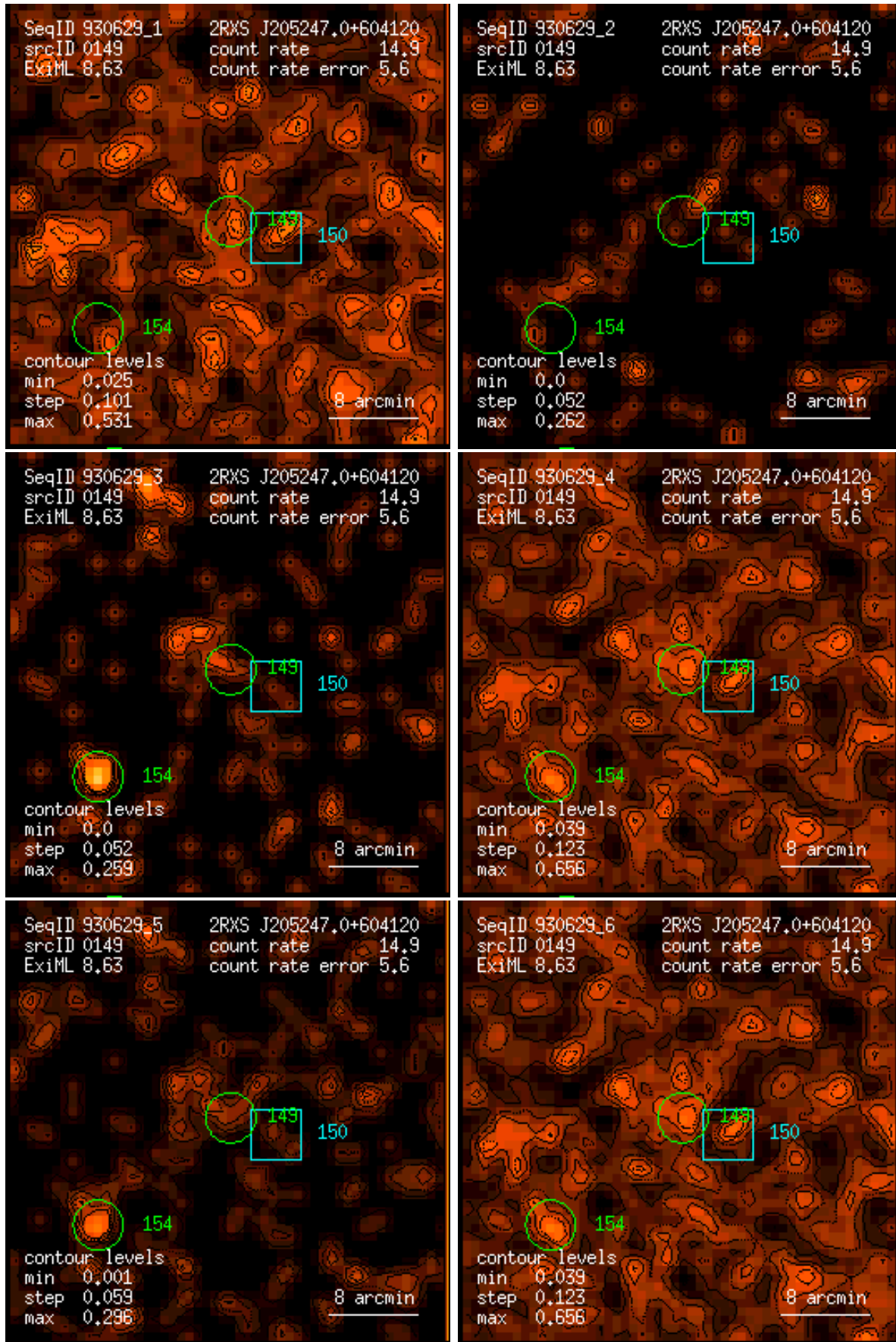
Figure 149: RASS 930629: detection 0149: band rate images, Gaussian filter: (1) PSPC channels 11 – 41, (2) 52 – 90, (3) 91 – 201, (4) 11 – 235, (5) 52 – 201, (6) 11 – 201. Broad band rates in counts/ks. Band rate contour levels in counts/ks/arcmin 2 .
