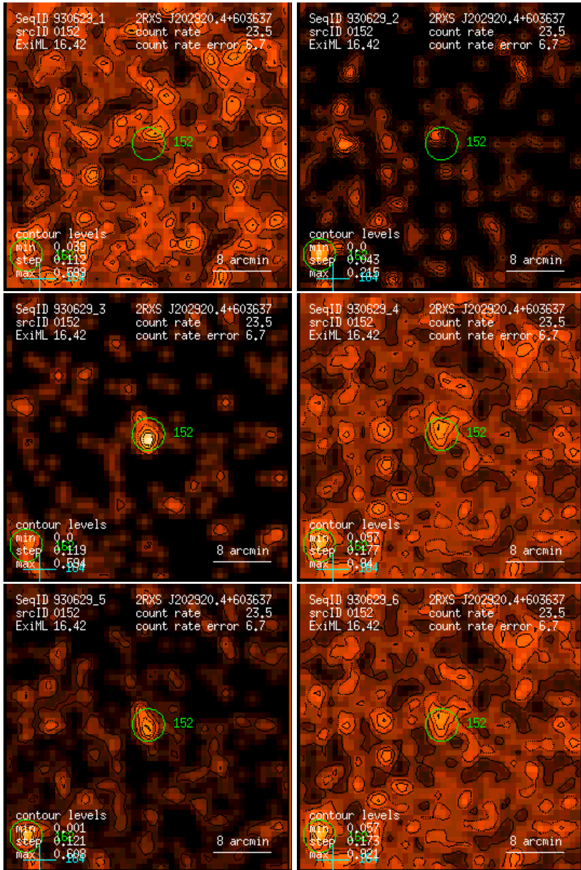
Figure 152: RASS 930629: detection 0152: band rate images, Gaussian filter: (1) PSPC channels 11 – 41, (2) 52 – 90, (3) 91 – 201, (4) 11 – 235, (5) 52 – 201, (6) 11 – 201. Broad band rates in counts/ks. Band rate contour levels in counts/ks/arcmin 2 .
