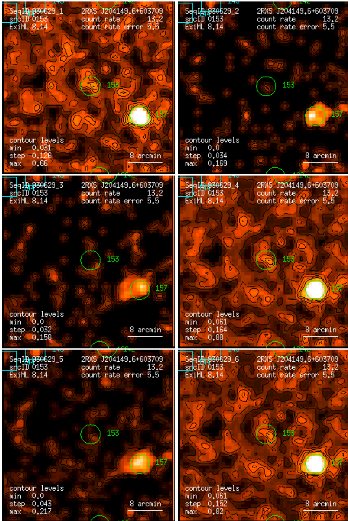
Figure 153: RASS 930629: detection 0153: band rate images, Gaussian filter: (1) PSPC channels 11 – 41, (2) 52 – 90, (3) 91 – 201, (4) 11 – 235, (5) 52 – 201, (6) 11 – 201. Broad band rates in counts/ks. Band rate contour levels in counts/ks/arcmin 2 .
