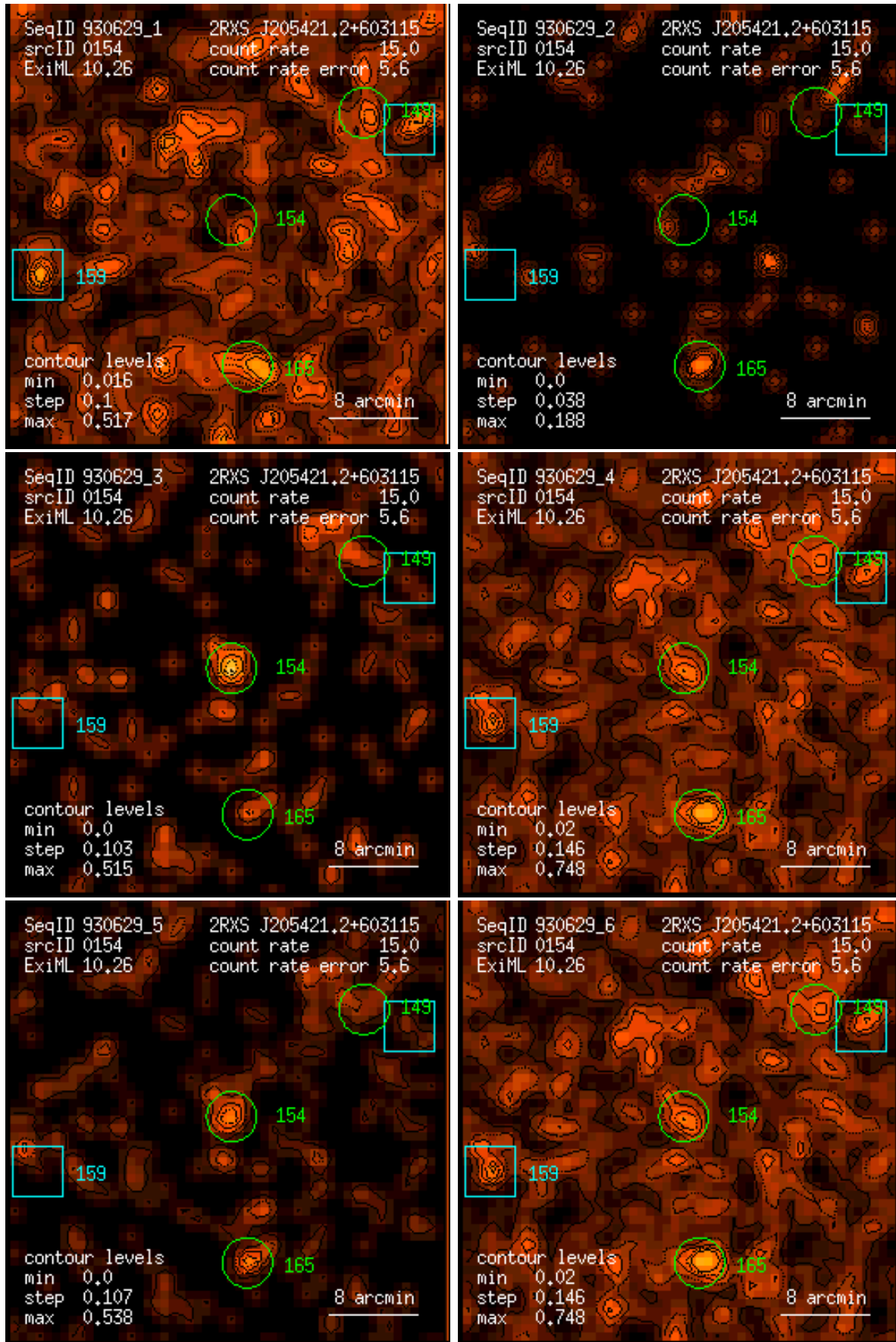
Figure 154: RASS 930629: detection 0154: band rate images, Gaussian filter: (1) PSPC channels 11 – 41, (2) 52 – 90, (3) 91 – 201, (4) 11 – 235, (5) 52 – 201, (6) 11 – 201. Broad band rates in counts/ks. Band rate contour levels in counts/ks/arcmin 2 .
