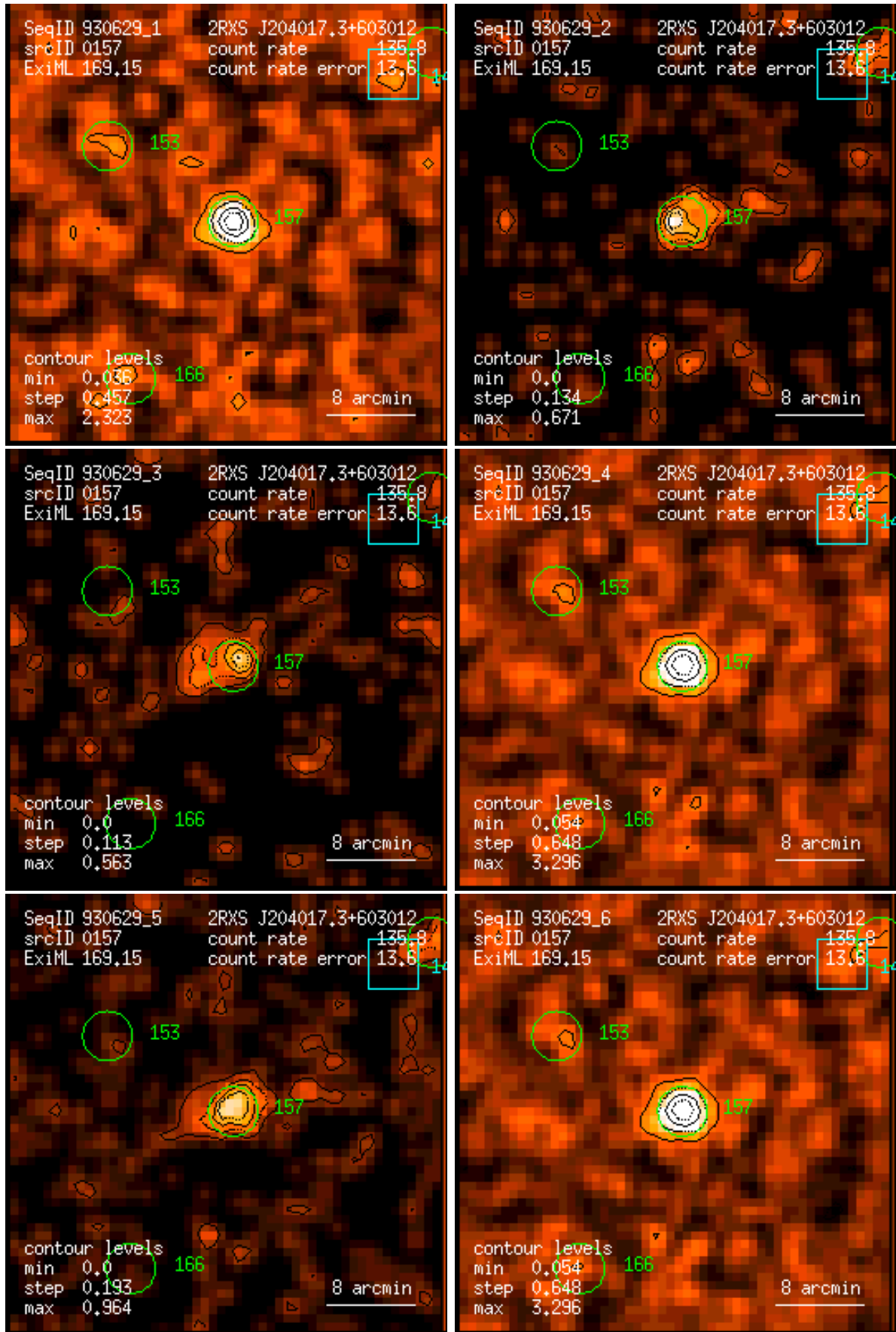
Figure 157: RASS 930629: detection 0157: band rate images, Gaussian filter: (1) PSPC channels 11 – 41, (2) 52 – 90, (3) 91 – 201, (4) 11 – 235, (5) 52 – 201, (6) 11 – 201. Broad band rates in counts/ks. Band rate contour levels in counts/ks/arcmin 2 .
