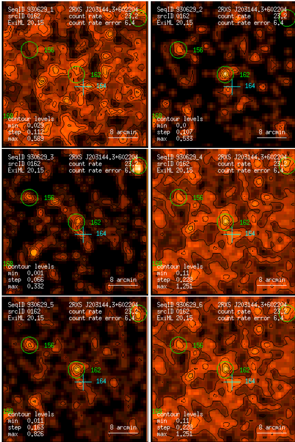
Figure 162: RASS 930629: detection 0162: band rate images, Gaussian filter: (1) PSPC channels 11 – 41, (2) 52 – 90, (3) 91 – 201, (4) 11 – 235, (5) 52 – 201, (6) 11 – 201. Broad band rates in counts/ks. Band rate contour levels in counts/ks/arcmin 2 .
