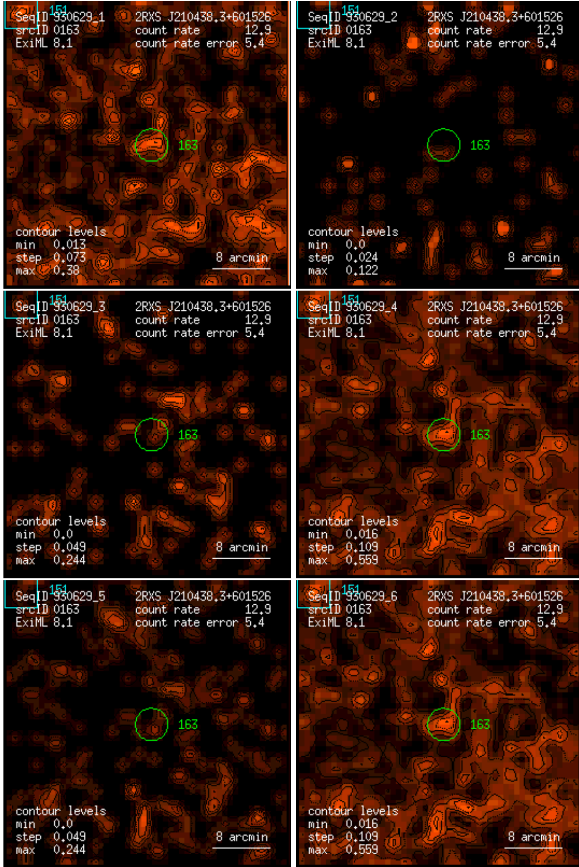
Figure 163: RASS 930629: detection 0163: band rate images, Gaussian filter: (1) PSPC channels 11 – 41, (2) 52 – 90, (3) 91 – 201, (4) 11 – 235, (5) 52 – 201, (6) 11 – 201. Broad band rates in counts/ks. Band rate contour levels in counts/ks/arcmin 2 .
