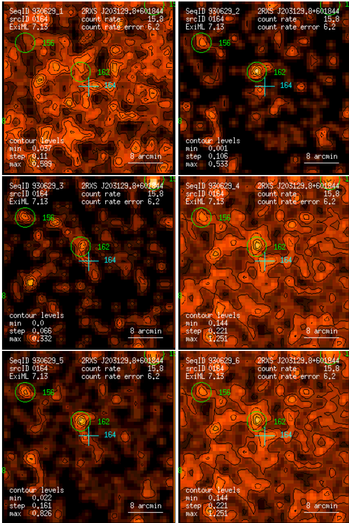
Figure 164: RASS 930629: detection 0164: band rate images, Gaussian filter: (1) PSPC channels 11 – 41, (2) 52 – 90, (3) 91 – 201, (4) 11 – 235, (5) 52 – 201, (6) 11 – 201. Broad band rates in counts/ks. Band rate contour levels in counts/ks/arcmin 2 .
