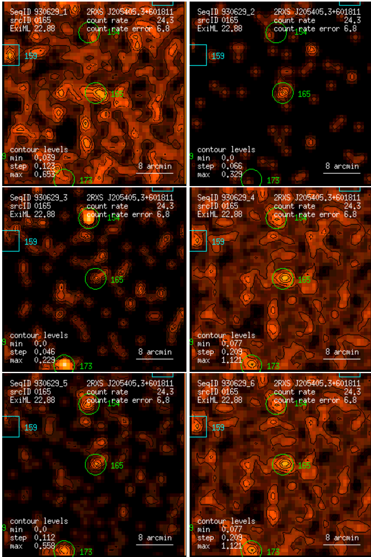
Figure 165: RASS 930629: detection 0165: band rate images, Gaussian filter: (1) PSPC channels 11 – 41, (2) 52 – 90, (3) 91 – 201, (4) 11 – 235, (5) 52 – 201, (6) 11 – 201. Broad band rates in counts/ks. Band rate contour levels in counts/ks/arcmin 2 .
